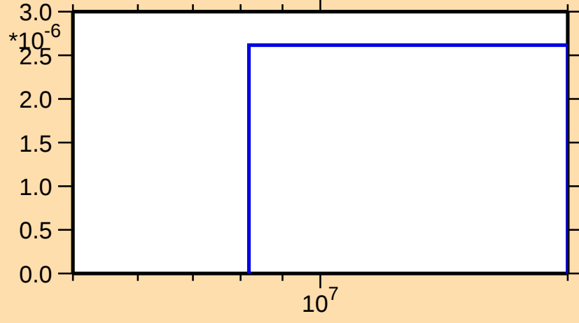
\sigma vs. E for ^{71}\text{Br}(n,2n)
