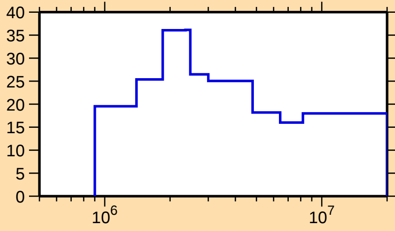
\Delta\sigma/\sigma vs. E for ^{71}\text{Br}(\text{n},\text{el.})
