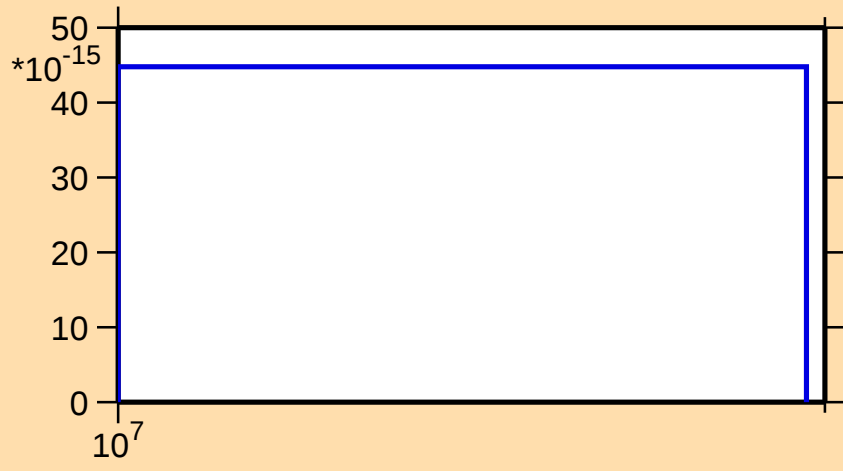
\sigma vs. E for ^{74}\text{Br}(n,\text{nt})
