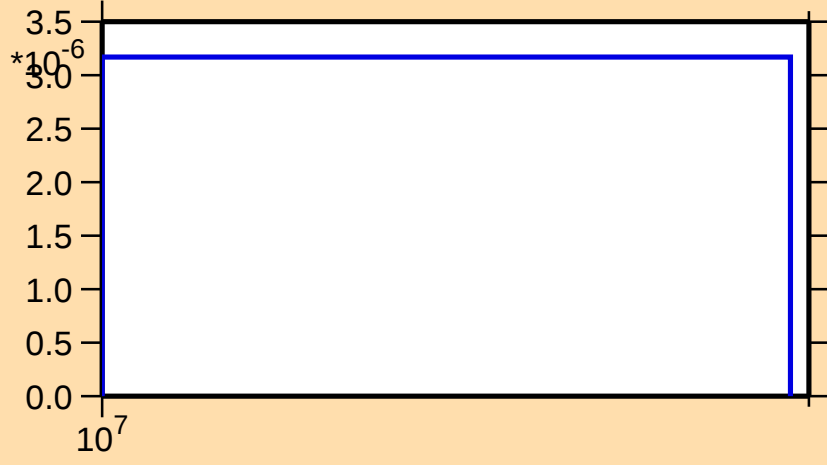
\sigma vs. E for ^{74}\text{Br}(n,\text{pd})
