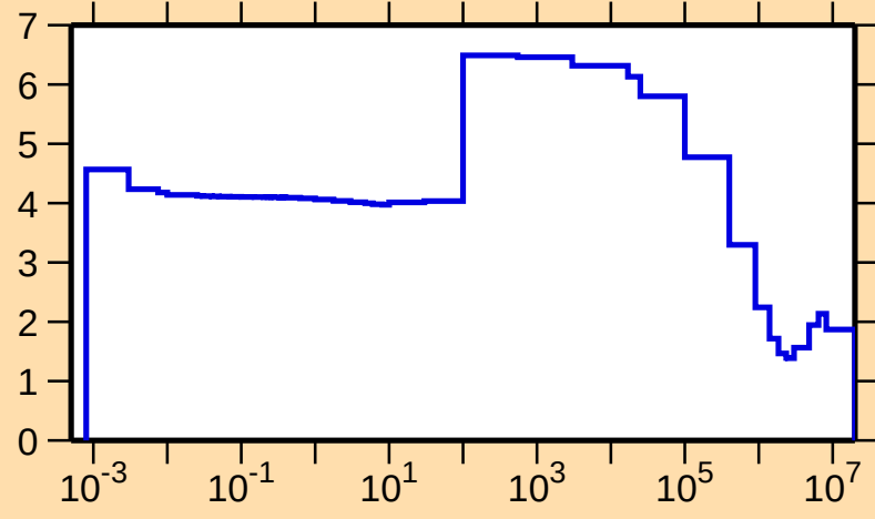
\sigma vs. E for ^{74}\text{Br}(n,\text{el.})
