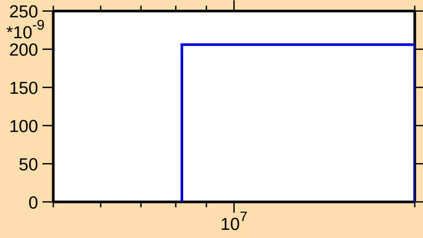
\sigma vs. E for ^{74}\text{Br}(\text{mt } 45)
