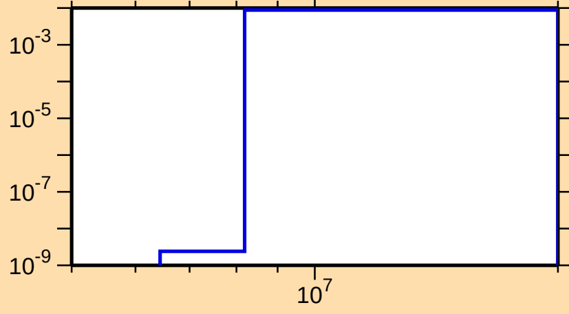
\sigma vs. E for ^{74}\text{Br}(n,\alpha)
