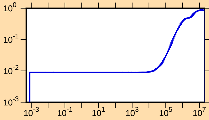
\mu vs. E for ^{75}\text{Br}(\text{mt251})
