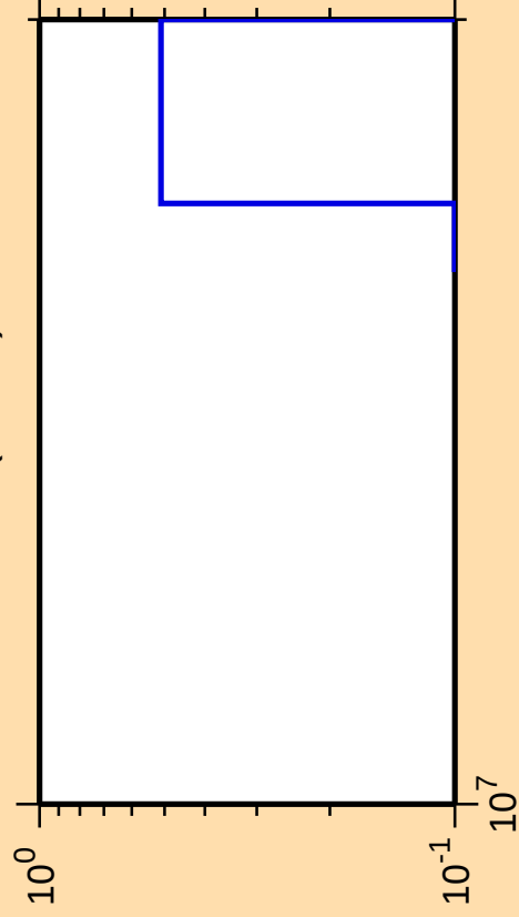
\Delta\sigma/\sigma vs. E for ^{75}\text{Br} (mt 34)
