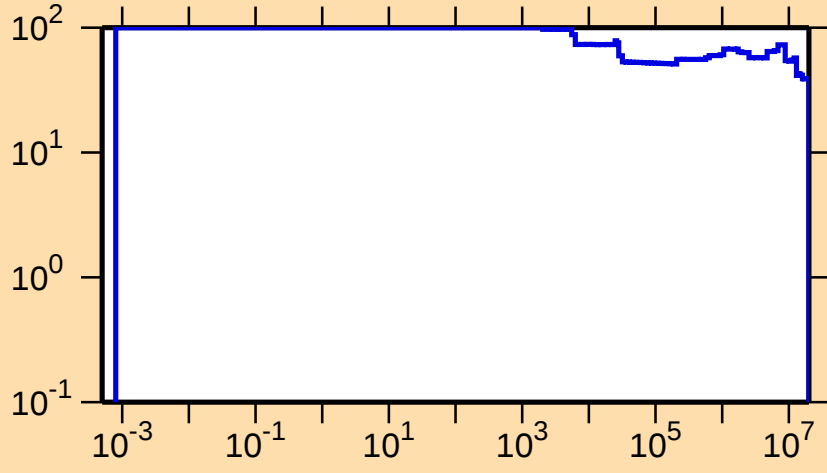
\Delta\sigma/\sigma vs. E for ^{75}\text{Br}(n,p)
