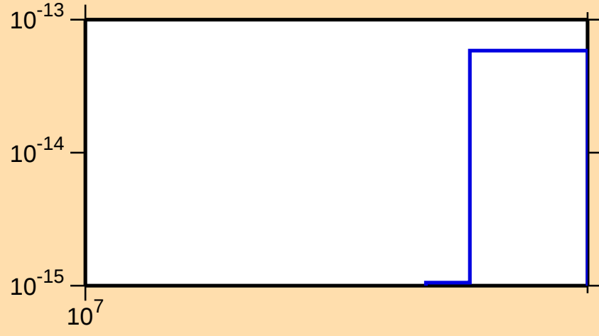
\sigma vs. E for ^{75}\text{Br} (mt 34)
