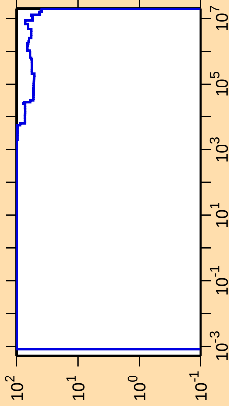
\Delta\sigma/\sigma vs. E for ^{75}\text{Br}(n,p)
