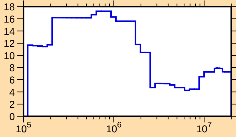
\Delta\sigma/\sigma vs. E for ^{75}\text{Br}(n,\text{tot.})
