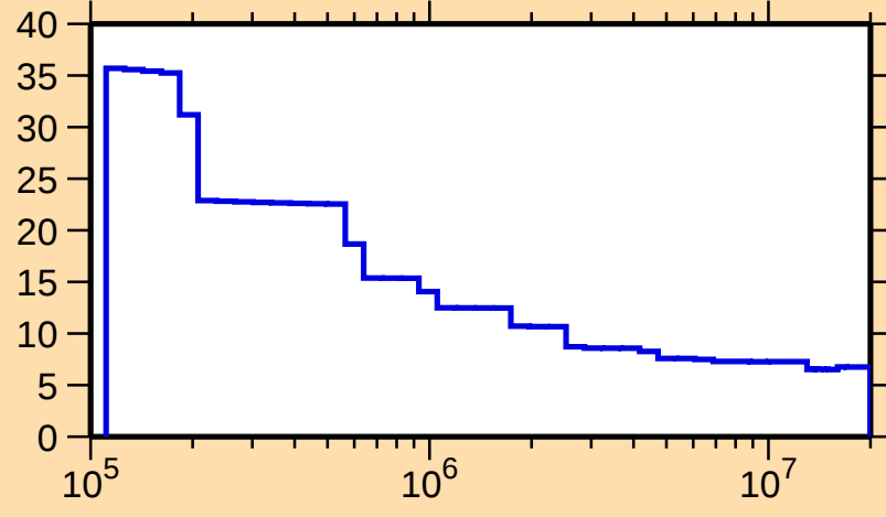
\Delta\sigma/\sigma vs. E for ^{75}\text{Br}(n,\text{nonel.})
