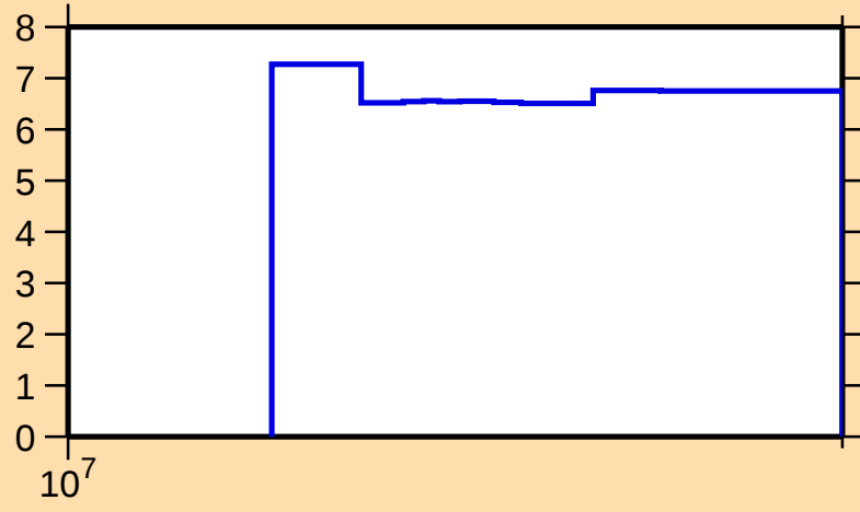
\Delta\sigma/\sigma vs. E for ^{75}\text{Br}(n,\text{nonel.})
