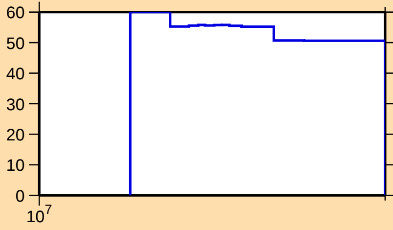
\Delta\sigma/\sigma vs. E for ^{75}\text{Br}(n,\text{inel.})
