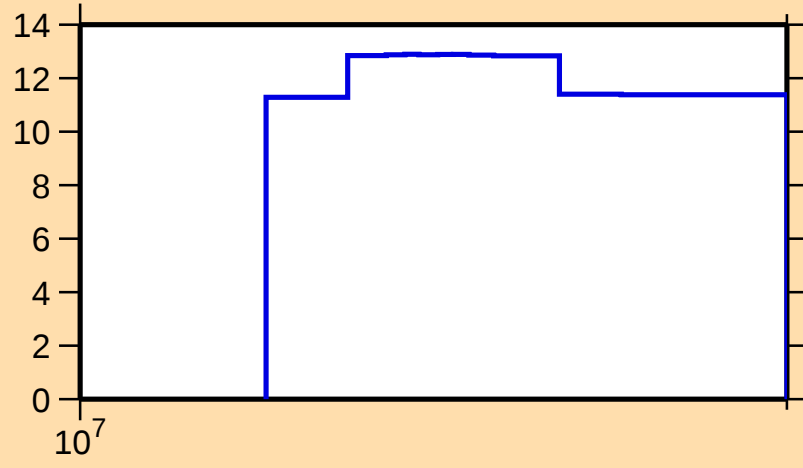
\Delta\sigma/\sigma vs. E for ^{75}\text{Br}(n,\text{el.})
