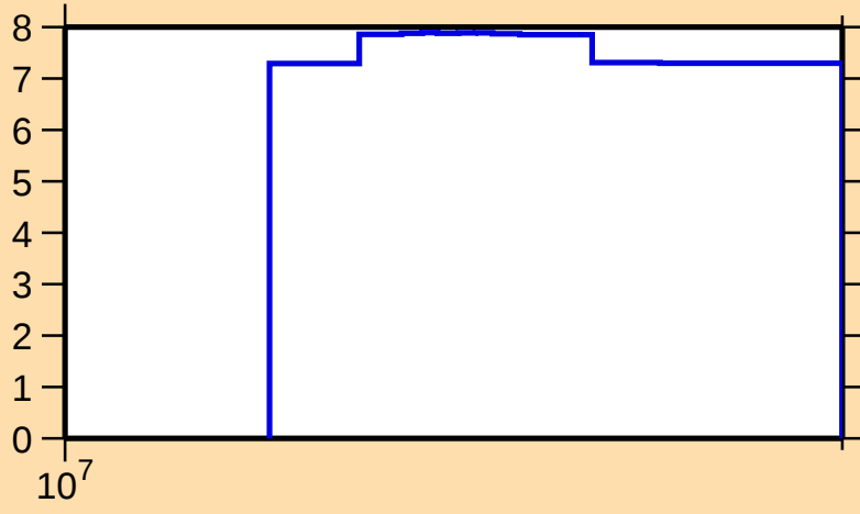
\Delta\sigma/\sigma vs. E for ^{75}\text{Br}(n,\text{tot.})
