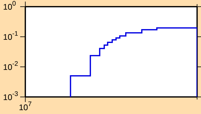
\sigma vs. E for ^{75}\text{Br}(n,2n)
