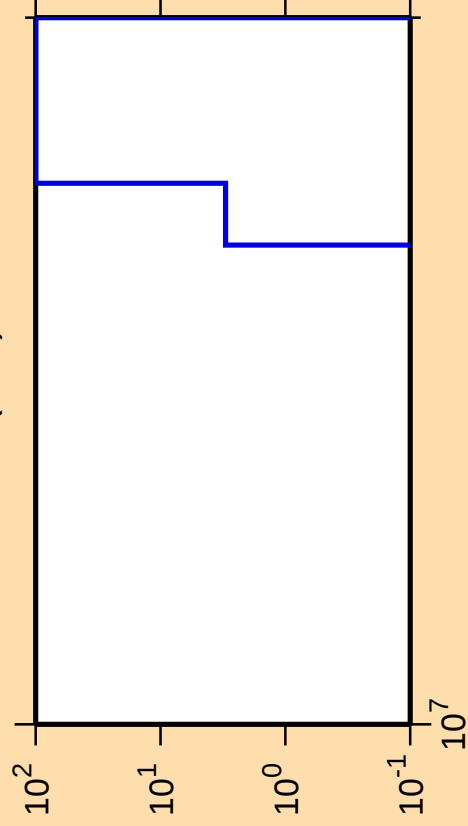
\Delta\sigma/\sigma vs. E for ^{75}\text{Br}(n,\text{nt})
