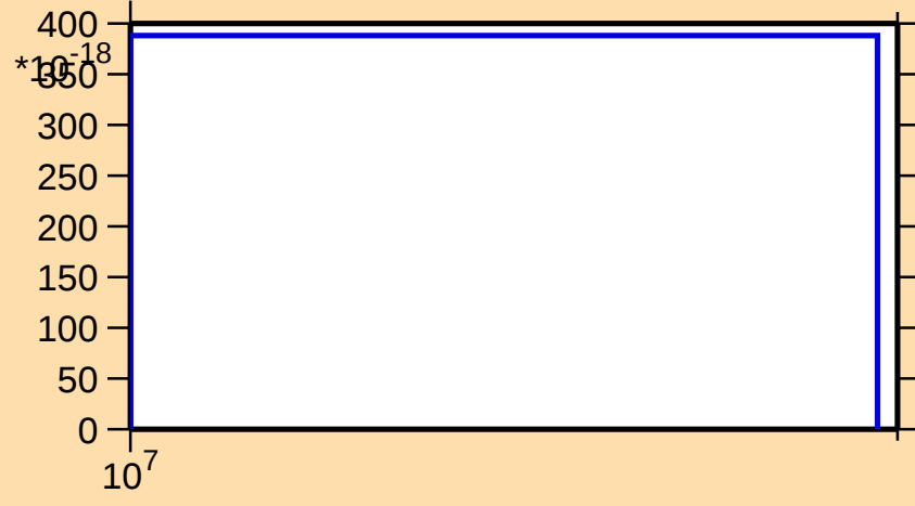
\sigma vs. E for ^{75}\text{Br} (mt 34)
