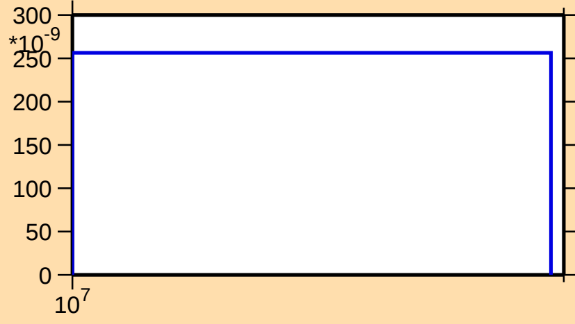
\sigma vs. E for ^{75}\text{Br}(n,\text{nd})
