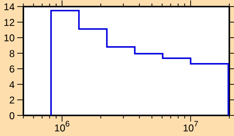
\Delta\sigma/\sigma vs. E for ^{75}\text{Br}(n,n\text{onel.})
