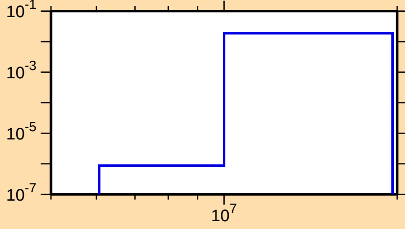
\sigma vs. E for ^{75}\text{Br}(n,\alpha)
