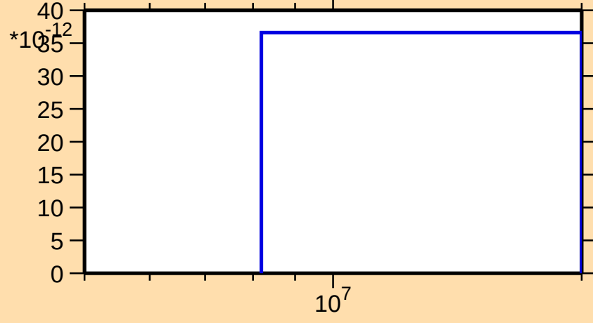
\sigma vs. E for ^{75}\text{Br}(n,\text{nt})
