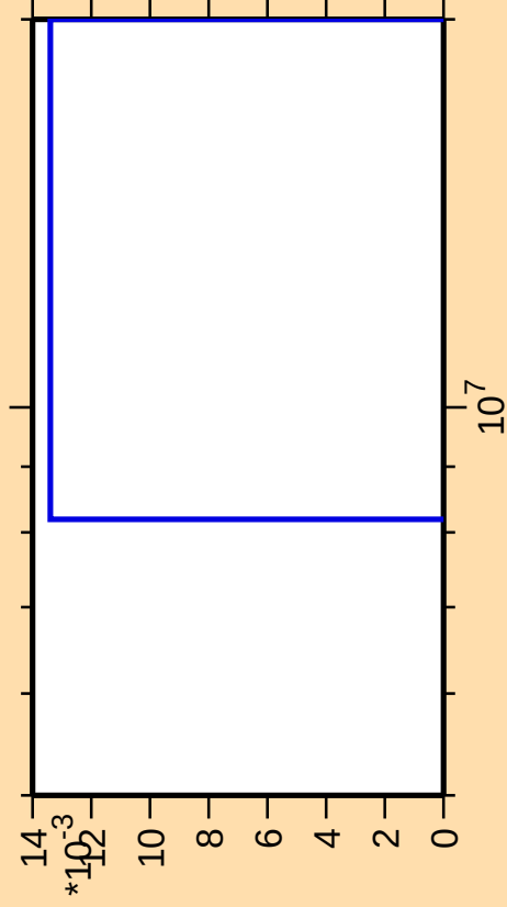
\Delta\sigma/\sigma vs. E for ^{75}\text{Br}(n,2n\alpha)
