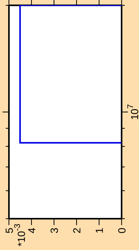
\Delta\sigma/\sigma vs. E for ^{75}\text{Br}(\text{mt } 34)
