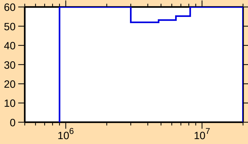
\Delta\sigma/\sigma vs. E for ^{75}\text{Br}(n,n\text{cont.})
