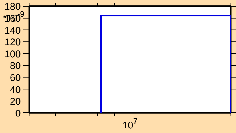
\sigma vs. E for ^{75}\text{Br}(\text{mt } 45)
