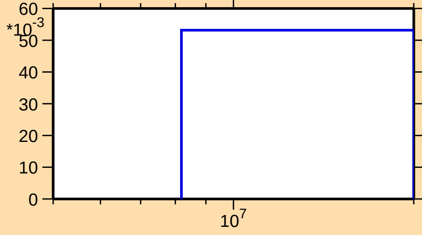
\sigma vs. E for ^{75}\text{Br}(n,2n)
