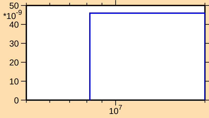
\sigma vs. E for ^{75}\text{Br}(\text{mt117})
