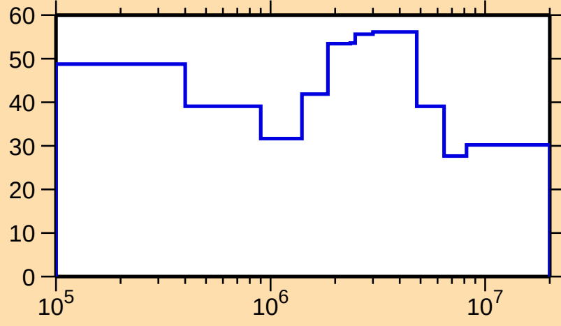
\Delta\sigma/\sigma vs. E for ^{75}\text{Br}(n,n_1)
