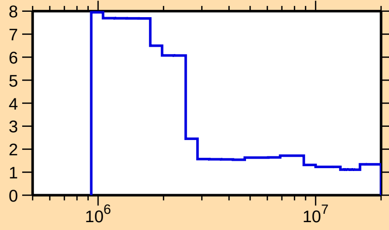
\Delta\sigma/\sigma vs. E for ^{77}\text{Br}(n,n\text{onel.})
