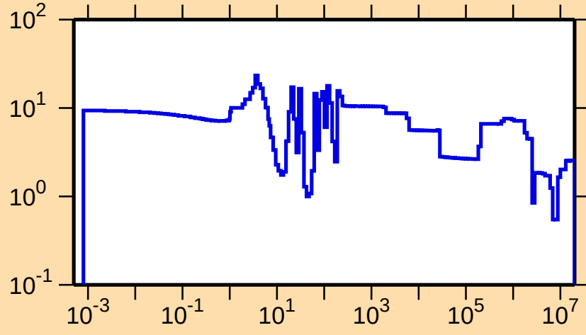
\Delta\sigma/\sigma vs. E for ^{77}\text{Br}(\text{n,tot.})
