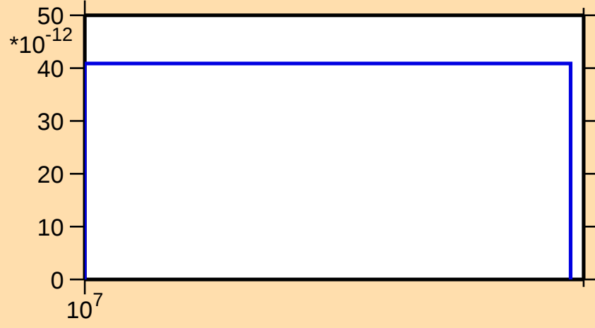
\sigma vs. E for ^{77}\text{Br}(n,\text{nt})
