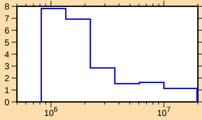
\Delta\sigma/\sigma vs. E for ^{77}\text{Br}(\text{n},\text{nonel.})
