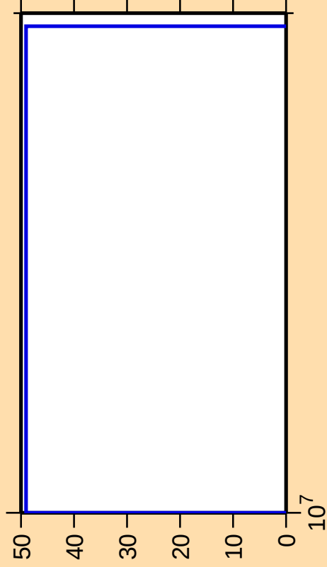
\Delta\sigma/\sigma vs. E for ^{77}\text{Br}(n,\text{nt})
