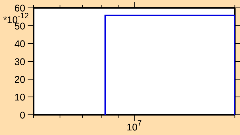
\sigma vs. E for ^{77}\text{Br}(n,\text{nt})
