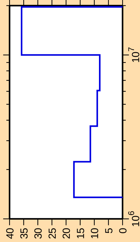
\Delta\sigma/\sigma vs. E for ^{81}\text{Br}(\text{n},\text{ncont.})
