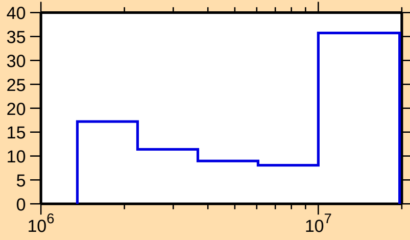
\Delta\sigma/\sigma vs. E for ^{81}\text{Br}(n,n\text{cont.})
