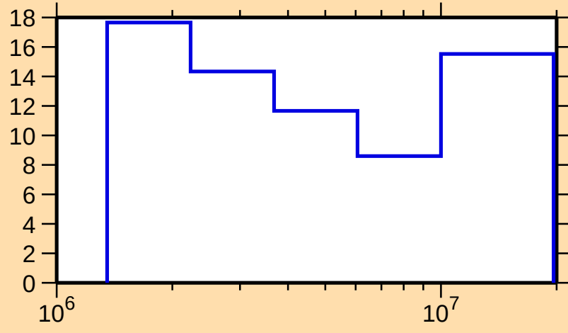
\Delta\sigma/\sigma vs. E for ^{81}\text{Br}(\text{n},\text{el.})
