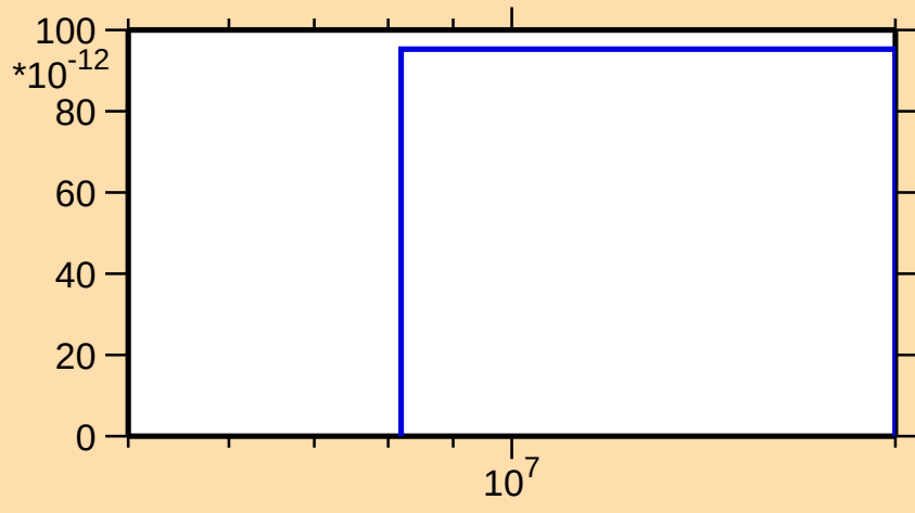
\sigma vs. E for ^{81}\text{Br}(n,\text{nt})
