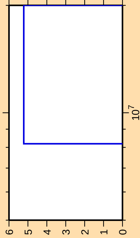
\Delta\sigma/\sigma vs. E for ^{81}\text{Br}(n,p\alpha)
