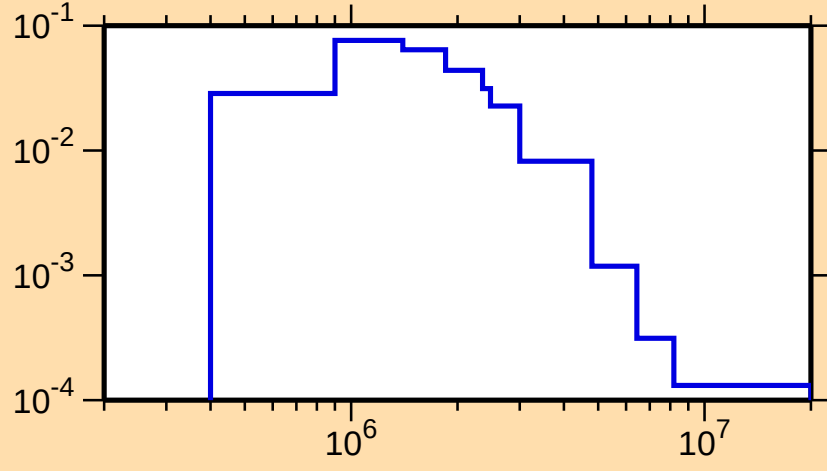
\sigma vs. E for ^{81}\text{Br}(n,n_2)
