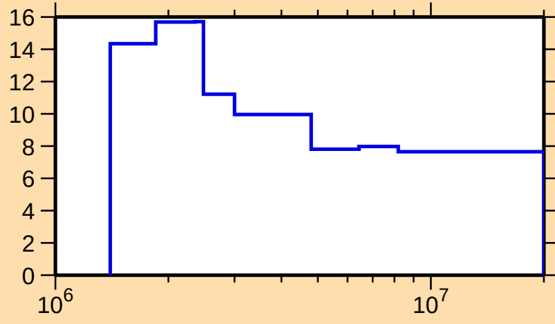
\Delta\sigma/\sigma vs. E for ^{81}\text{Br}(n,n\text{oncl.})
