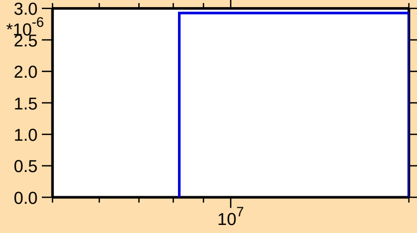
\sigma vs. E for ^{81}\text{Br}(n,3n)
