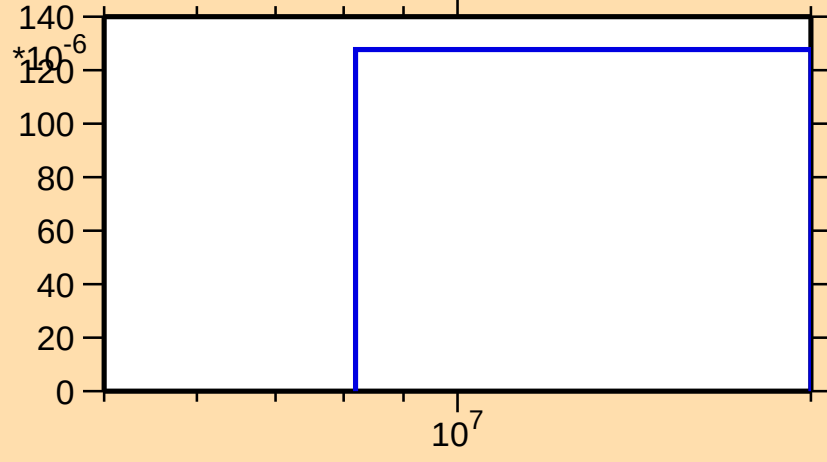
\sigma vs. E for ^{81}\text{Br}(n,n\alpha)
