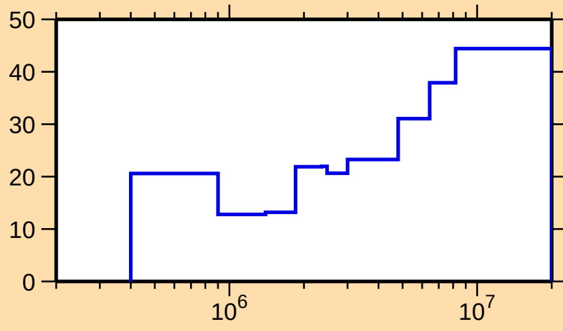
\Delta\sigma/\sigma vs. E for ^{81}\text{Br}(n,n_1)
