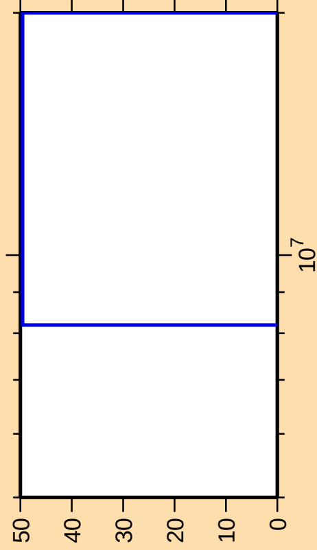
\Delta\sigma/\sigma vs. E for ^{81}\text{Br}(n,n\alpha)
