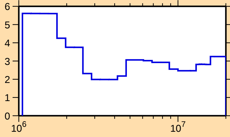
\Delta\sigma/\sigma vs. E for ^{82}\text{Br}(n,n\text{onel.})
