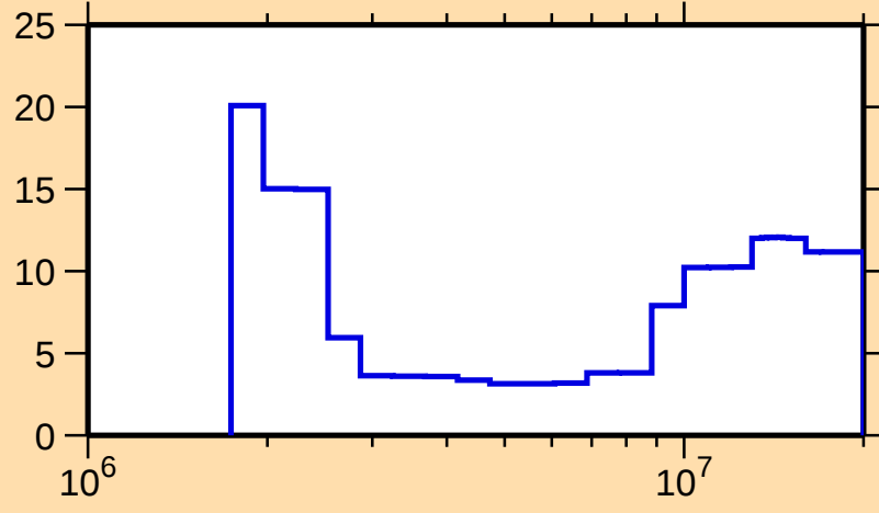
\Delta\sigma/\sigma vs. E for ^{82}\text{Br}(n,n\text{cont.})
