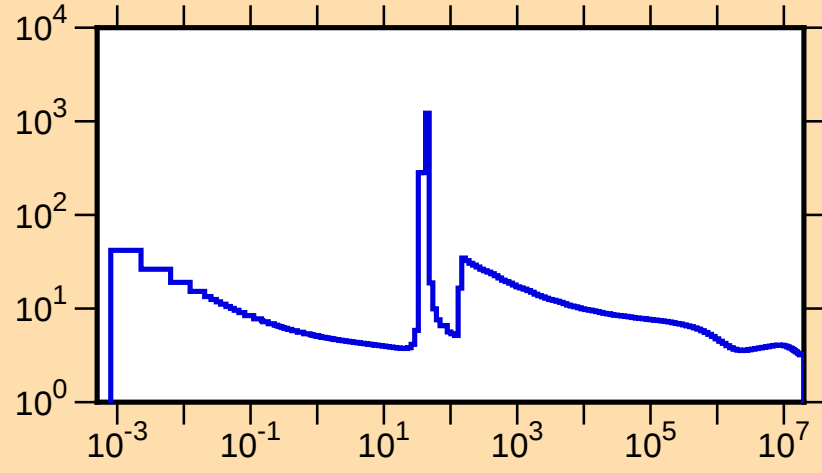
\sigma vs. E for ^{82}\text{Br}(n,\text{tot.})
