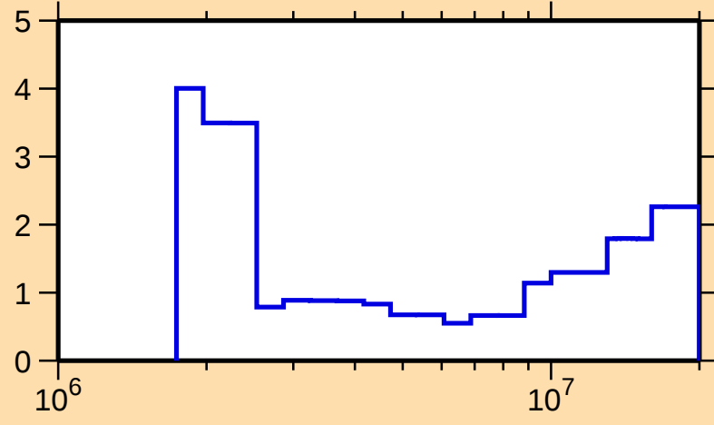
\Delta\sigma/\sigma vs. E for ^{82}\text{Br}(n,\text{tot.})
