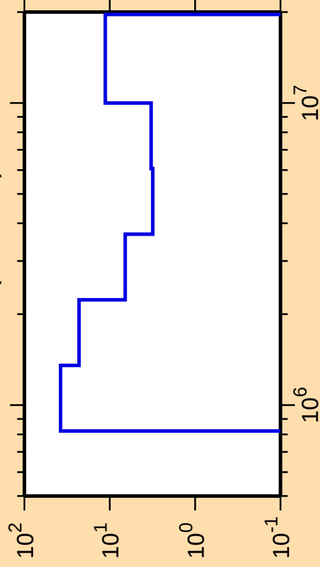
\Delta\sigma/\sigma vs. E for ^{82}\text{Br}(n,\text{ncont.})
