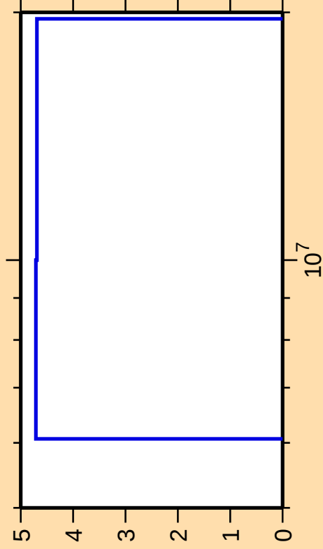
\Delta\sigma/\sigma vs. E for ^{82}\text{Br}(n,2n)
