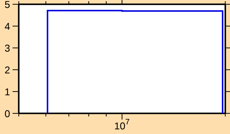
\Delta\sigma/\sigma vs. E for ^{82}\text{Br}(n,2n)
