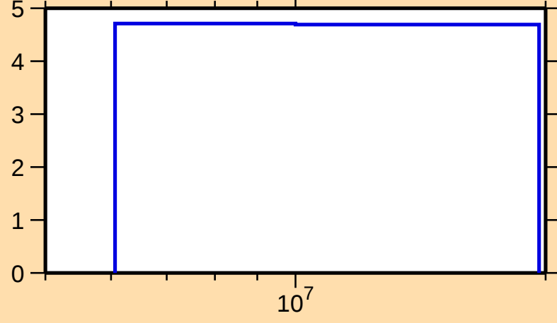
\Delta\sigma/\sigma vs. E for ^{82}\text{Br}(n,2n)
