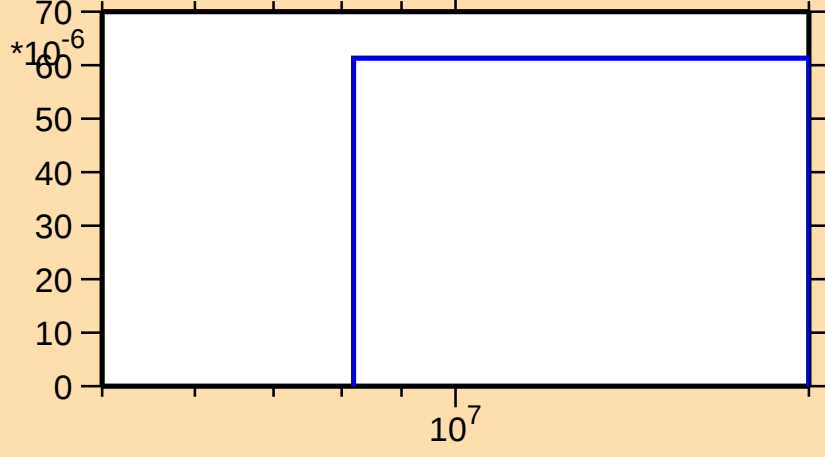
\sigma vs. E for ^{82}\text{Br}(n,\alpha)
