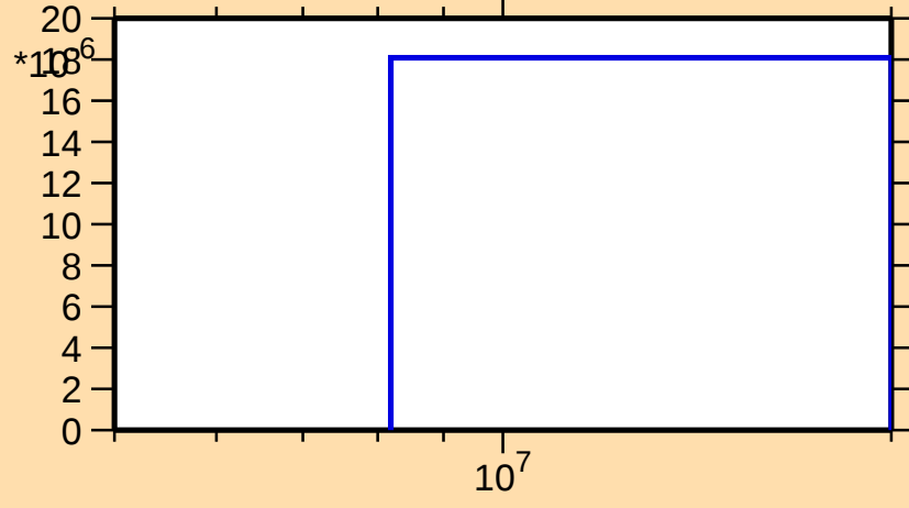
\sigma vs. E for ^{82}\text{Br}(n,3n)
