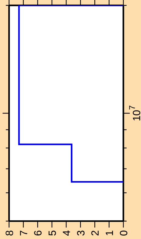
\Delta\sigma/\sigma vs. E for ^{82}\text{Br}(n,n\text{cont.})
