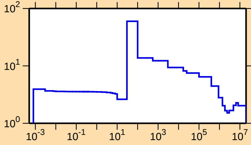
\sigma vs. E for ^{82}\text{Br}(n,\text{el.})
