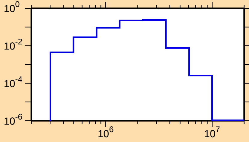
\sigma vs. E for ^{84}\text{Br}(n,n_1)
