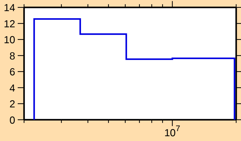
\Delta\sigma/\sigma vs. E for ^{84}\text{Br}(\text{n},\text{nonel.})
