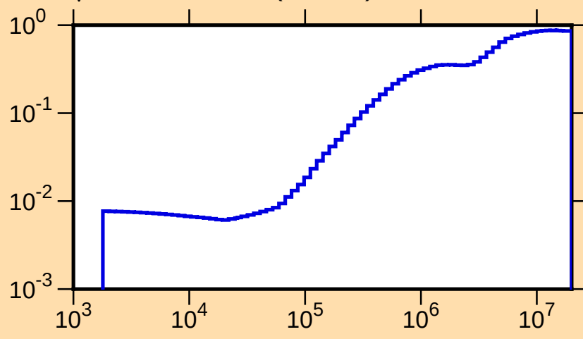
\mu vs. E for ^{85}\text{Br}(\text{mt251})
