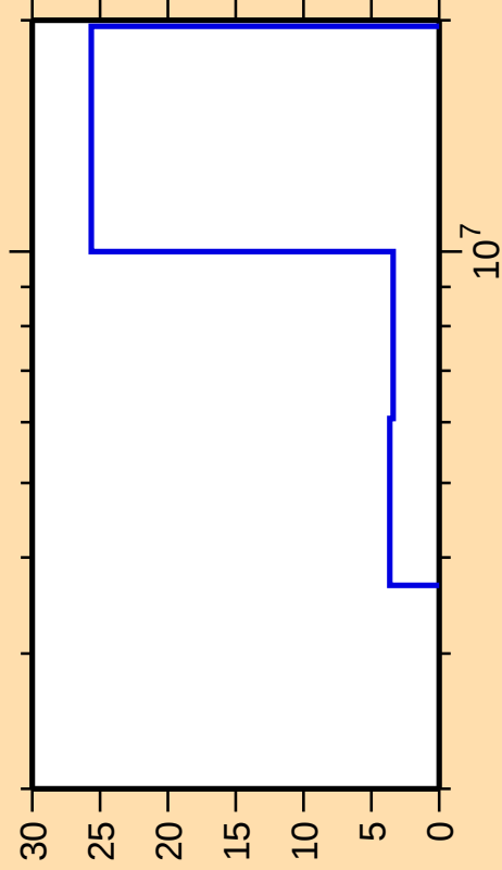
\Delta\sigma/\sigma vs. E for ^{85}\text{Br}(n,\text{ncont.})
