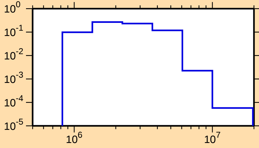
\sigma vs. E for ^{85}\text{Br}(n,n_2)
