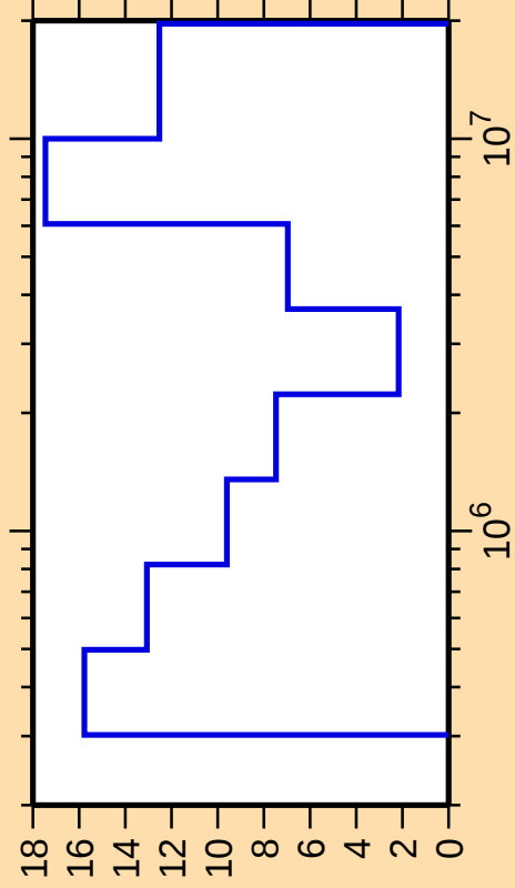
\Delta\sigma/\sigma vs. E for ^{85}\text{Br}(n,n_1)
