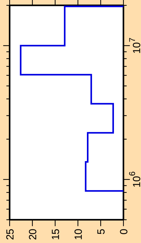
\Delta\sigma/\sigma vs. E for ^{85}\text{Br}(n,n_2)
