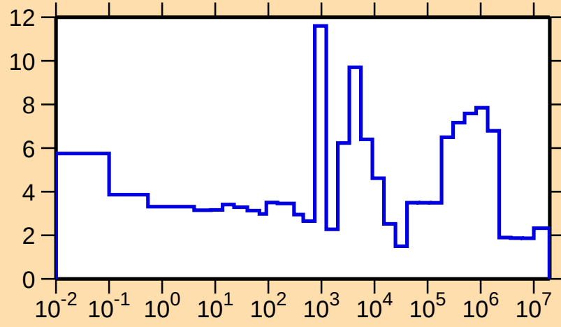
\Delta\sigma/\sigma vs. E for ^{85}\text{Br}(n,\text{tot.})
