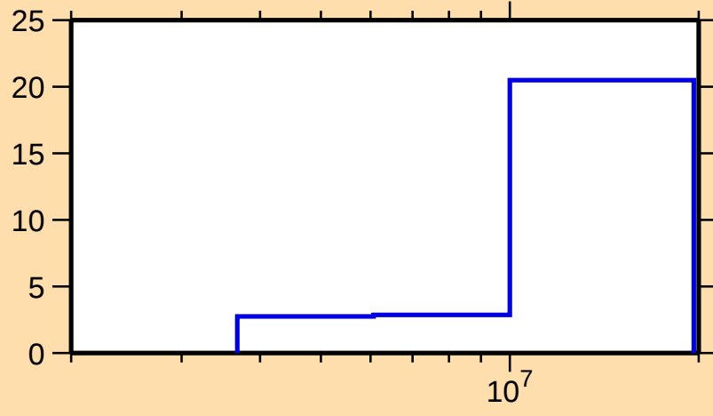
\Delta\sigma/\sigma vs. E for ^{85}\text{Br}(\text{n},\text{inel.})
