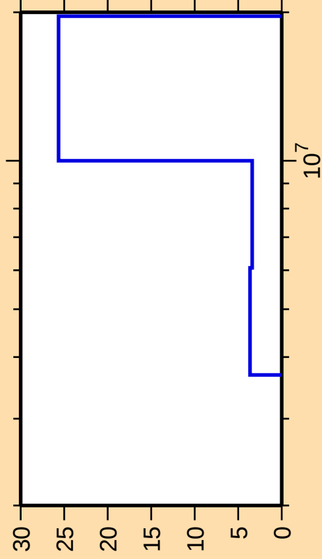
\Delta\sigma/\sigma vs. E for ^{85}\text{Br}(\text{n},\text{ncont.})
