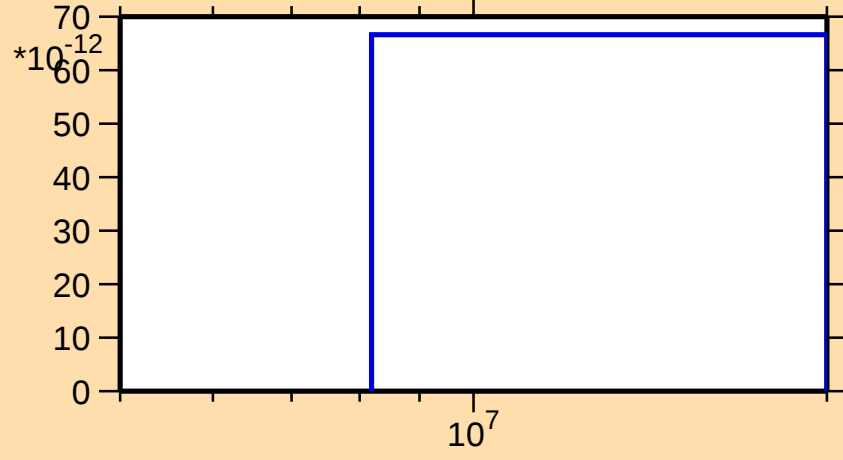
\sigma vs. E for ^{85}\text{Br}(n,\text{nt})
