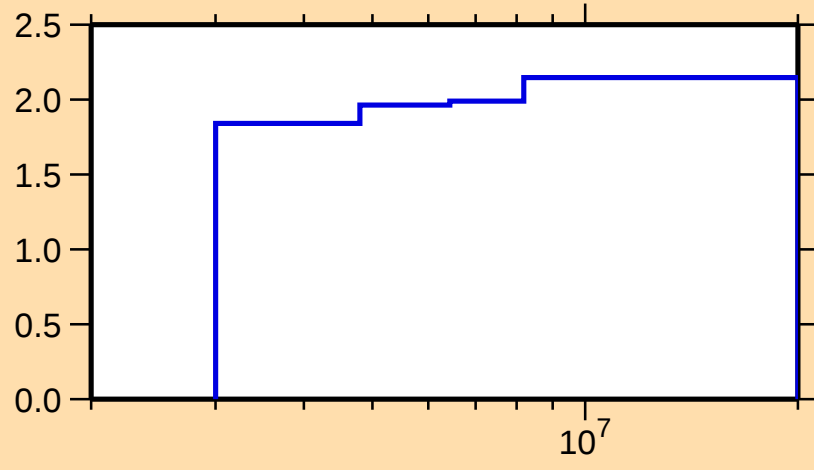
\Delta\sigma/\sigma vs. E for ^{85}\text{Br}(\text{n},\text{tot.})
