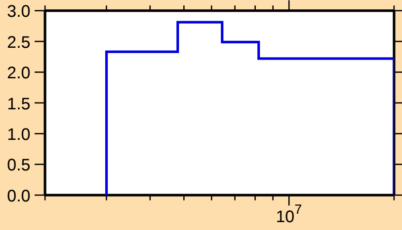
\Delta\sigma/\sigma vs. E for ^{85}\text{Br}(\text{n},\text{nonel.})
