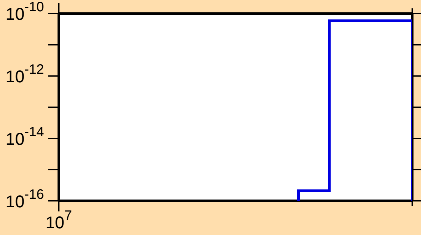
\sigma vs. E for ^{86}\text{Br}(n,2n\alpha)
