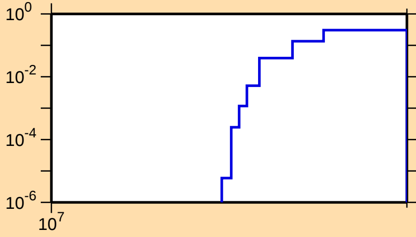
\sigma vs. E for ^{86}\text{Br}(n,3n)
