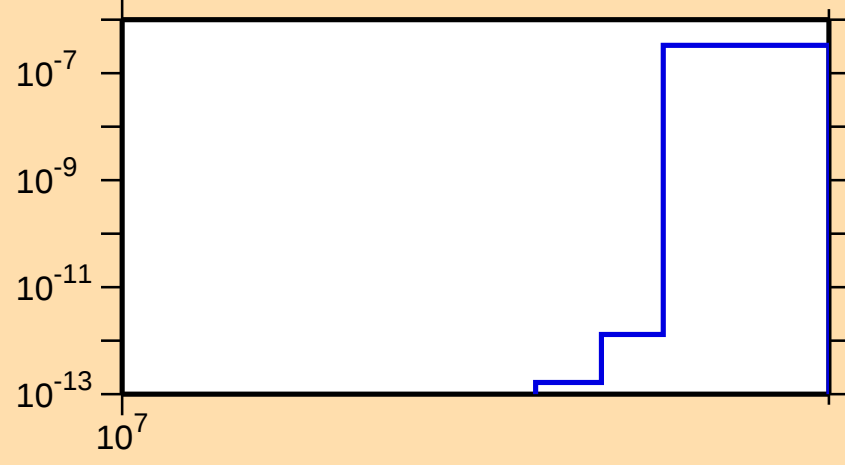
\sigma vs. E for ^{86}\text{Br}(n,\text{nt})
