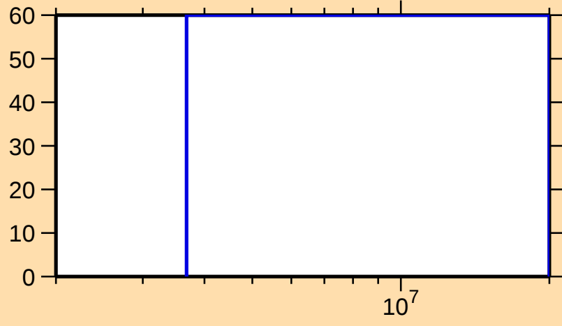
\Delta\sigma/\sigma vs. E for ^{86}\text{Br}(n,n_1)
