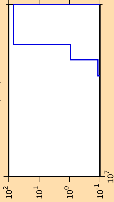
\Delta\sigma/\sigma vs. E for ^{86}\text{Br}(n,\text{nt})
