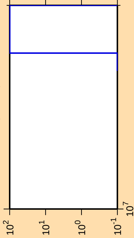
\Delta\sigma/\sigma vs. E for ^{86}\text{Br}(n,2n\alpha)
