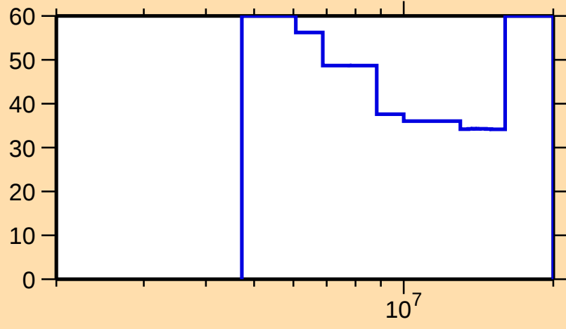
\Delta\sigma/\sigma vs. E for ^{86}\text{Br}(n,2n)
