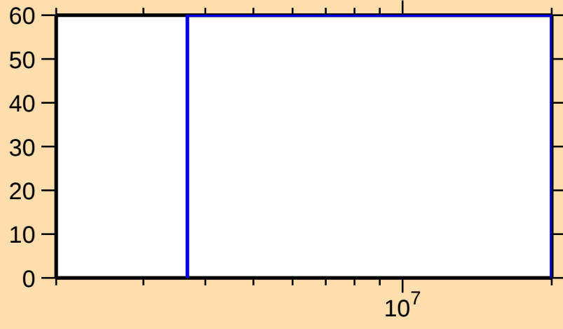
\Delta\sigma/\sigma vs. E for ^{86}\text{Br}(n,n\text{cont.})
