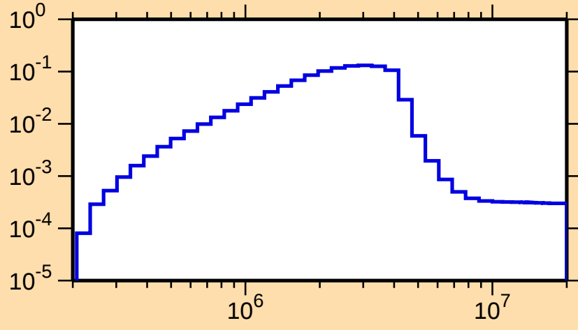
\sigma vs. E for ^{86}\text{Br}(n,n_4)
