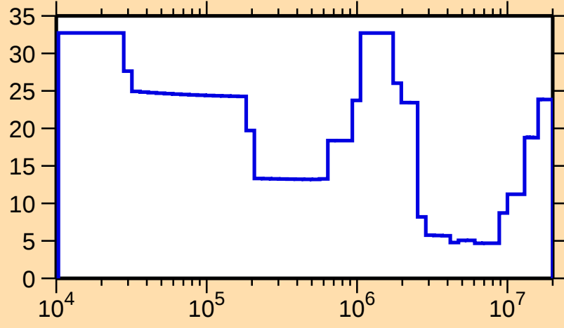
\Delta\sigma/\sigma vs. E for ^{86}\text{Br}(n,\text{tot.})
