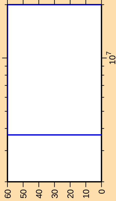
\Delta\sigma/\sigma vs. E for ^{86}\text{Br}(n,n\text{cont.})
