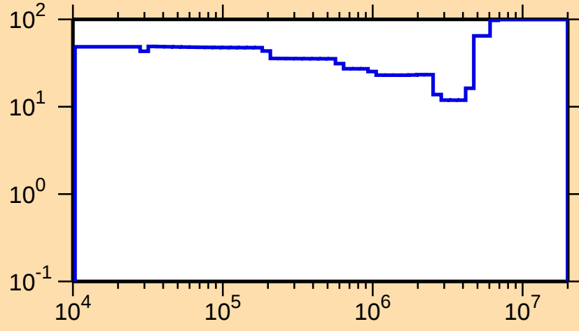
\Delta\sigma/\sigma vs. E for ^{86}\text{Br}(n,\text{inel.})
