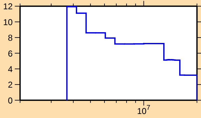
\Delta\sigma/\sigma vs. E for ^{86}\text{Br}(n,\text{nonel.})
