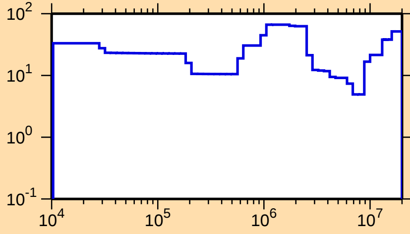
\Delta\sigma/\sigma vs. E for ^{86}\text{Br}(n,\text{el.})
