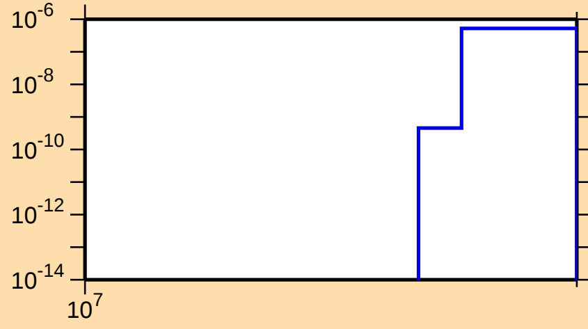
\sigma vs. E for ^{86}\text{Br}(n,2np)
