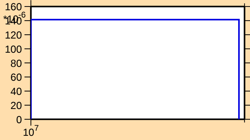
\sigma vs. E for ^{86}\text{Br}(n,np)
