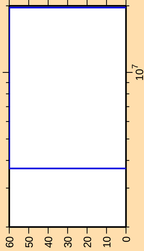
\Delta\sigma/\sigma vs. E for ^{86}\text{Br}(\text{n},\text{ncont.})
