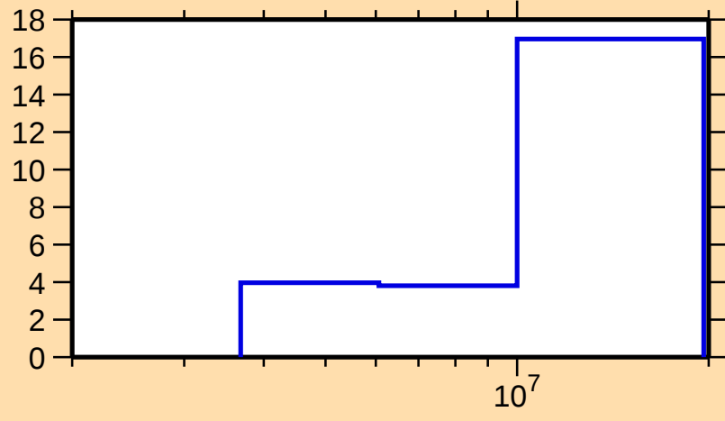
\Delta\sigma/\sigma vs. E for ^{86}\text{Br}(\text{n},\text{tot.})
