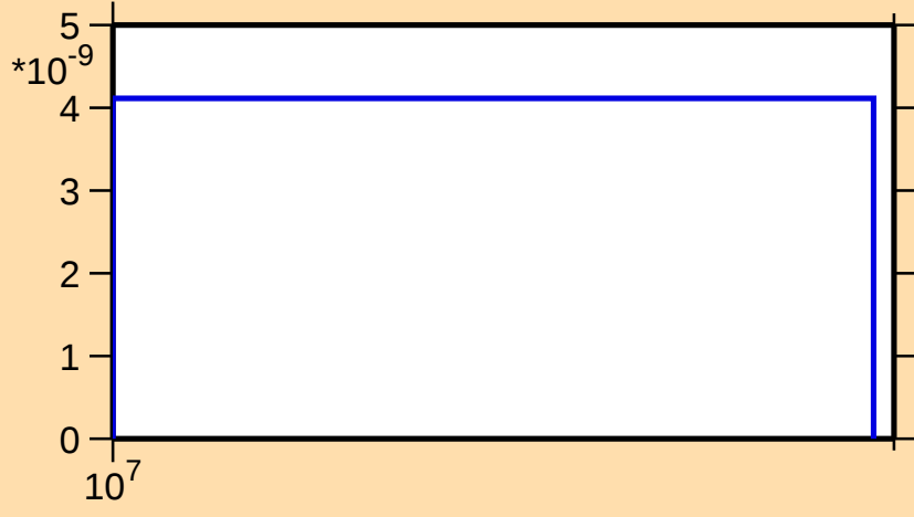
\sigma vs. E for ^{86}\text{Br}(n,2np)
