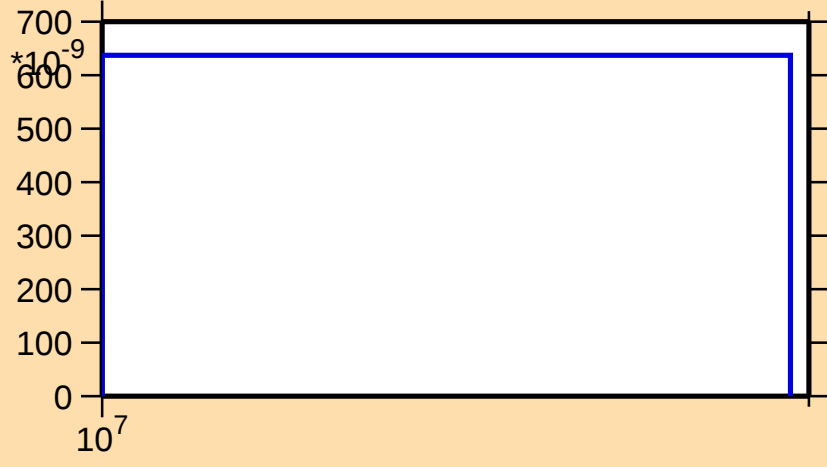
\sigma vs. E for ^{86}\text{Br}(n,\text{nd})
