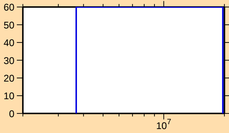
\Delta\sigma/\sigma vs. E for ^{86}\text{Br}(n,p)
