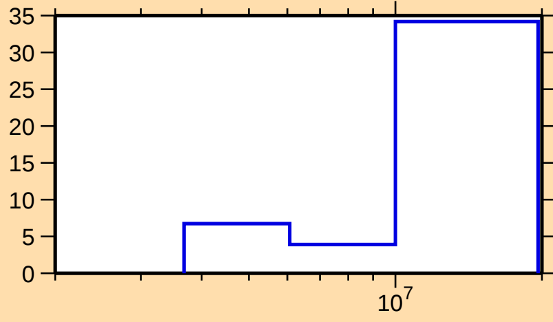
\Delta\sigma/\sigma vs. E for ^{86}\text{Br}(n,\text{el.})
