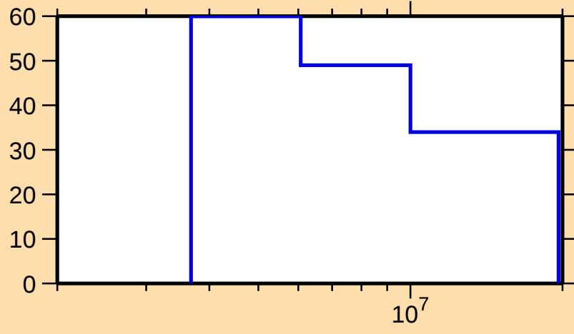
\Delta\sigma/\sigma vs. E for ^{86}\text{Br}(n,2n)
