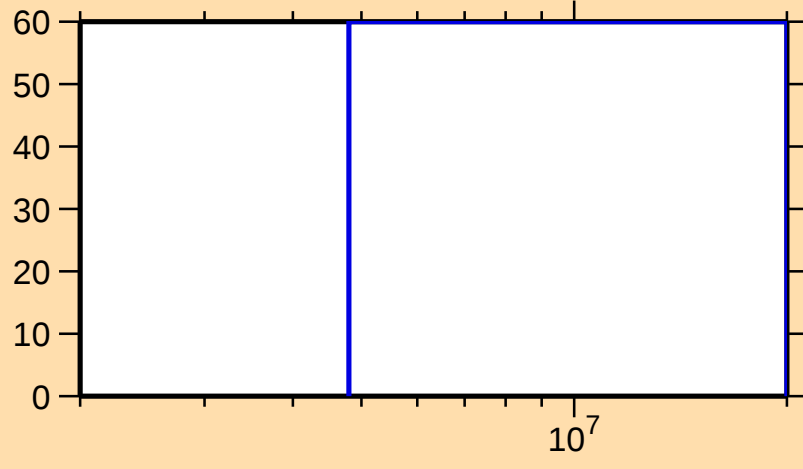
\Delta\sigma/\sigma vs. E for ^{86}\text{Br}(n,\text{inel.})
