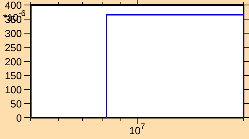
\sigma vs. E for ^{86}\text{Br}(n,d)
