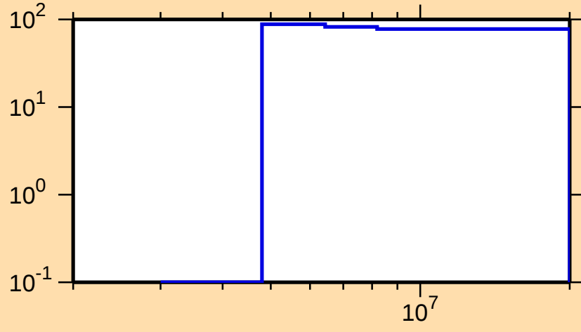
\Delta\sigma/\sigma vs. E for ^{86}\text{Br}(n,p)
