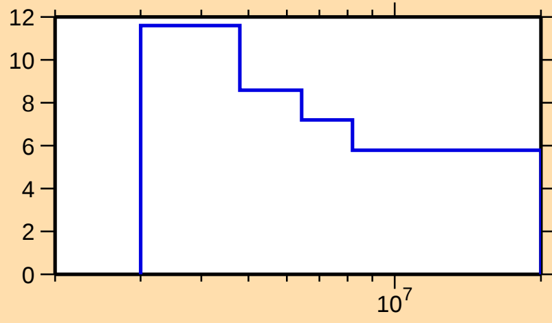
\Delta\sigma/\sigma vs. E for ^{86}\text{Br}(\text{n},\text{nonel.})
