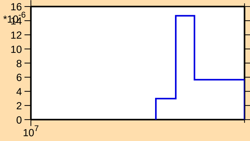
\sigma vs. E for ^{10}\text{C}(n,t)
