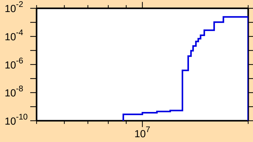
\sigma vs. E for ^{10}\text{C}(n,\alpha)
