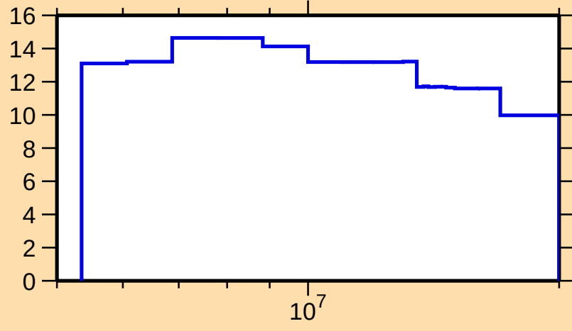
\Delta\sigma/\sigma vs. E for ^{10}\text{C}(\text{n},\text{el.})
