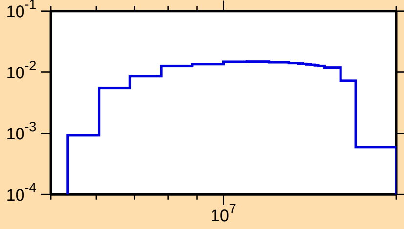
\sigma vs. E for ^{10}\text{C}(\text{n,ncont.})
