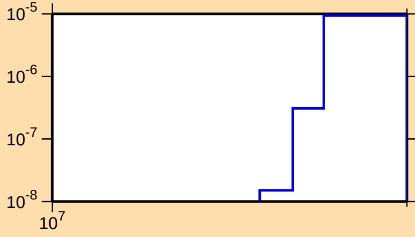
\sigma vs. E for ^{10}\text{C}(\text{n},\text{pt})
