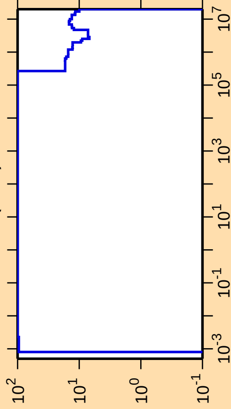
\Delta\sigma/\sigma vs. E for ^{10}\text{C}(\text{n,el.})
