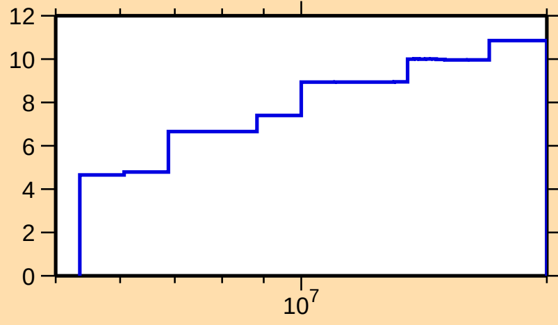
\Delta\sigma/\sigma vs. E for ^{10}\text{C}(\text{n},\text{nonel.})
