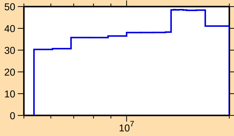
\Delta\sigma/\sigma vs. E for ^{10}\text{C}(\text{n,inel.})
