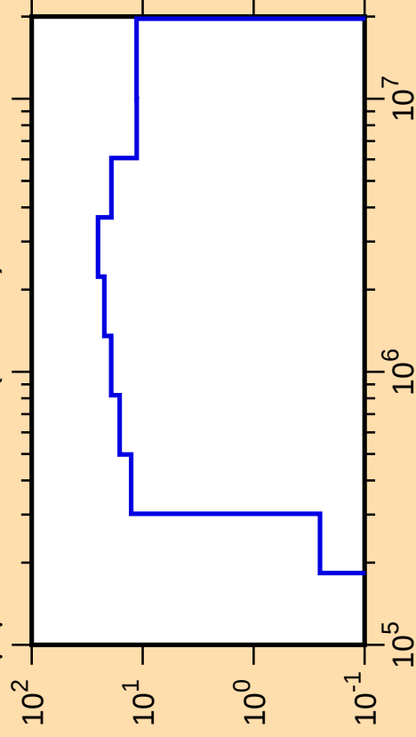
\Delta\mu/\mu vs. E for ^{10}\text{C}(\text{mt251})
