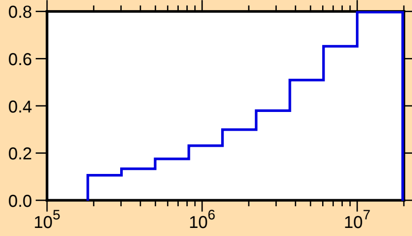
\mu vs. E for ^{10}\text{C}(\text{mt251})
