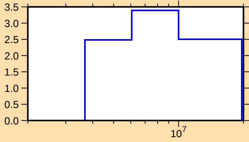
\Delta\sigma/\sigma vs. E for ^{10}\text{C}(\text{n},\text{tot.})
