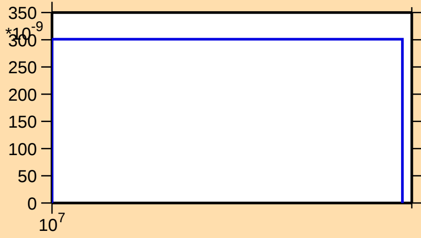
\sigma vs. E for ^{10}\text{C}(\text{mt } 34)
