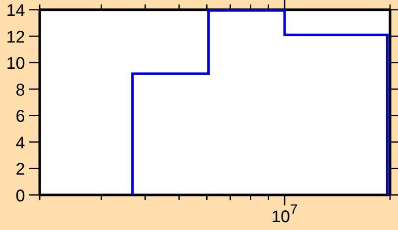
\Delta\sigma/\sigma vs. E for ^{10}\text{C}(\text{n,el.})
