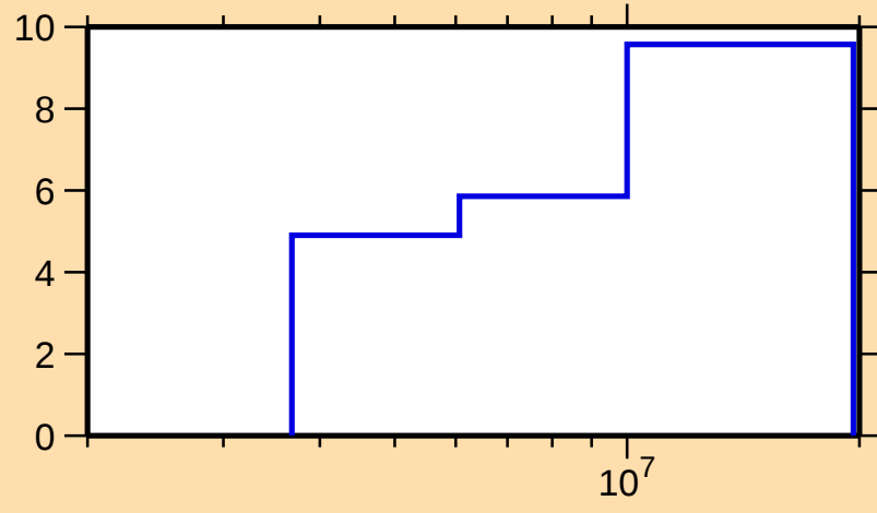
\Delta\sigma/\sigma vs. E for ^{10}\text{C}(\text{n,nonel.})
