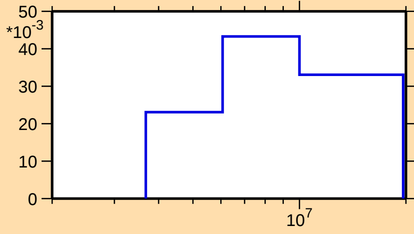
\sigma vs. E for ^{10}\text{C}(\text{n,inel.})
