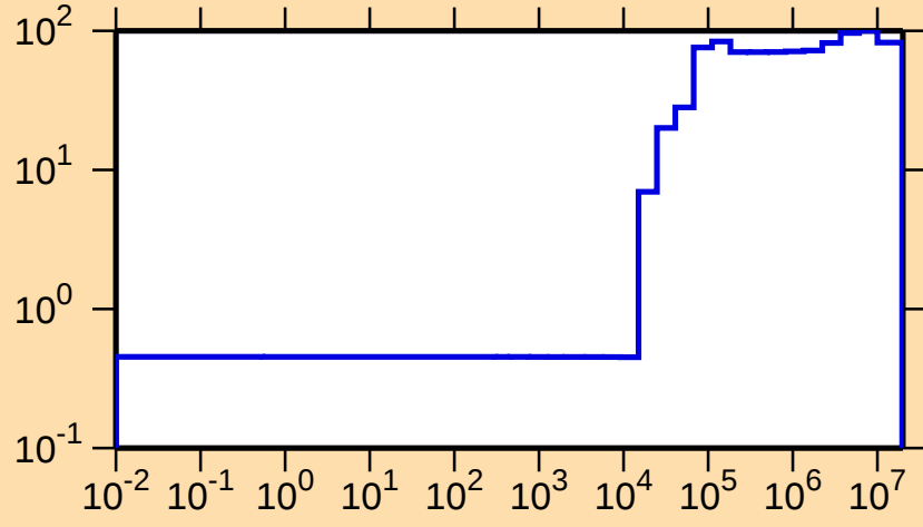
\Delta\sigma/\sigma vs. E for ^{10}\text{C}(n,\gamma)
