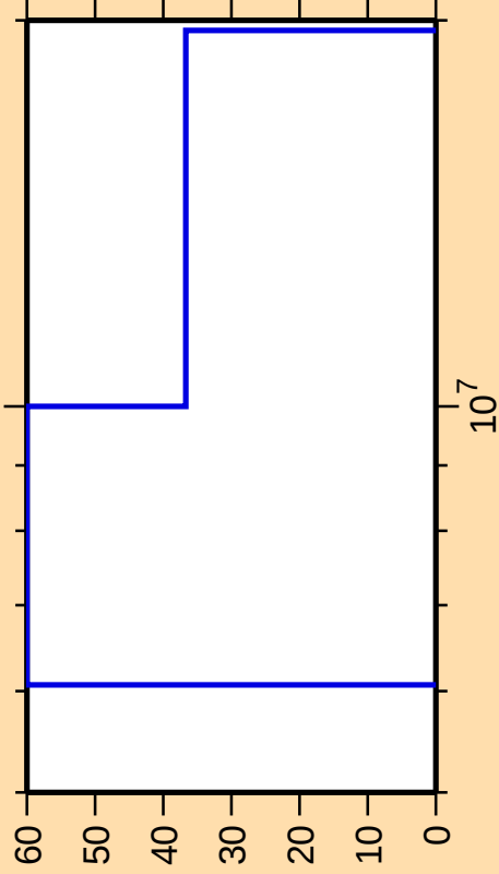
\Delta\sigma/\sigma vs. E for ^{10}\text{C}(\text{mt117})
