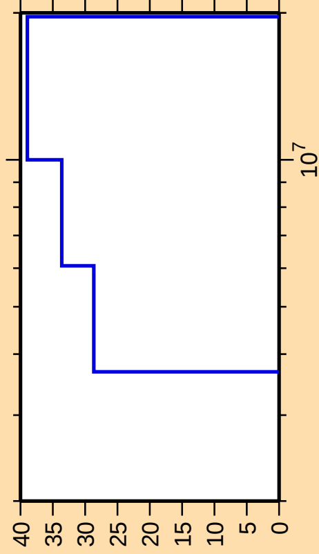
\Delta\sigma/\sigma vs. E for ^{10}\text{C}(\text{n,inel.})
