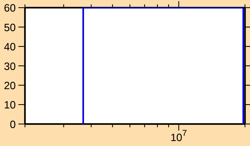
\Delta\sigma/\sigma vs. E for ^{10}\text{C}(n,n\text{cont.})
