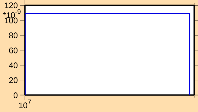
\sigma vs. E for ^{10}\text{C}(\text{n,pt})
