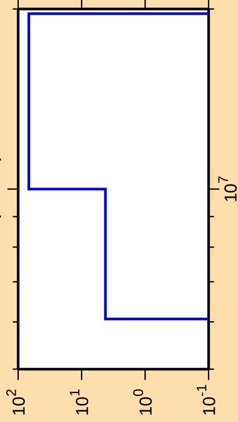
\Delta\sigma/\sigma vs. E for ^{10}\text{C}(\text{mt } 45)
