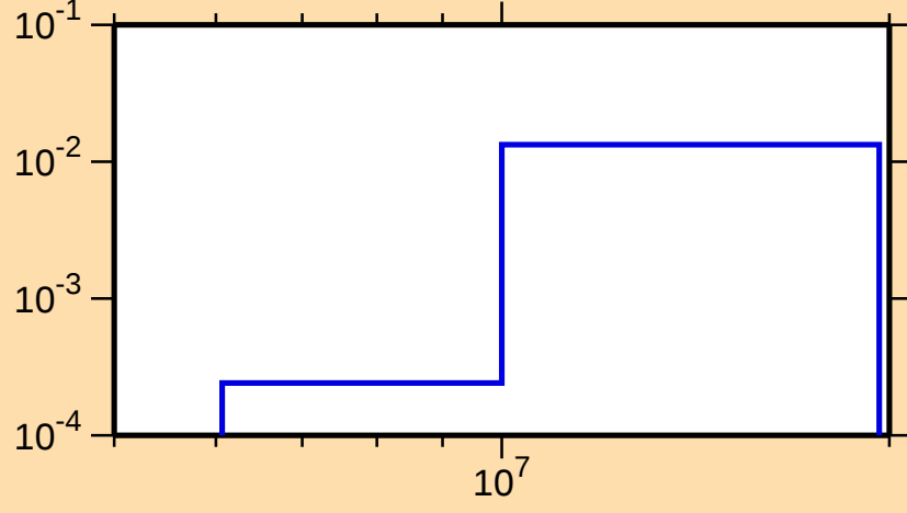
\sigma vs. E for ^{10}\text{C}(\text{mt117})
