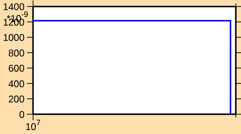
\sigma vs. E for ^{10}\text{C}(\text{n,t})
