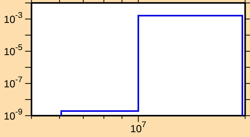
\sigma vs. E for ^{10}\text{C}(\text{mt } 45)
