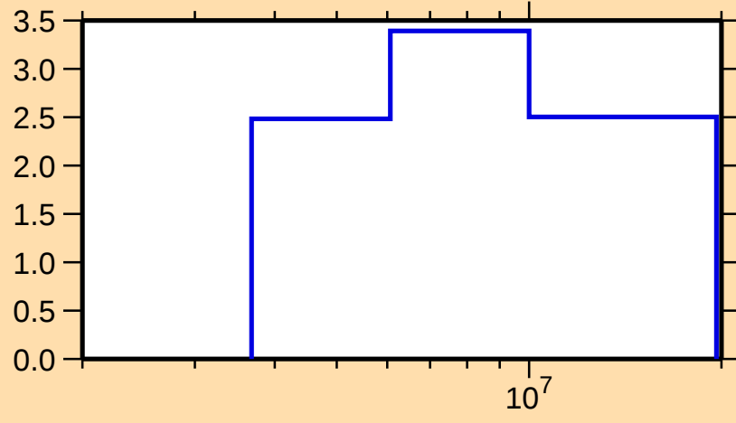
\Delta\sigma/\sigma vs. E for ^{10}\text{C}(\text{n,tot.})
