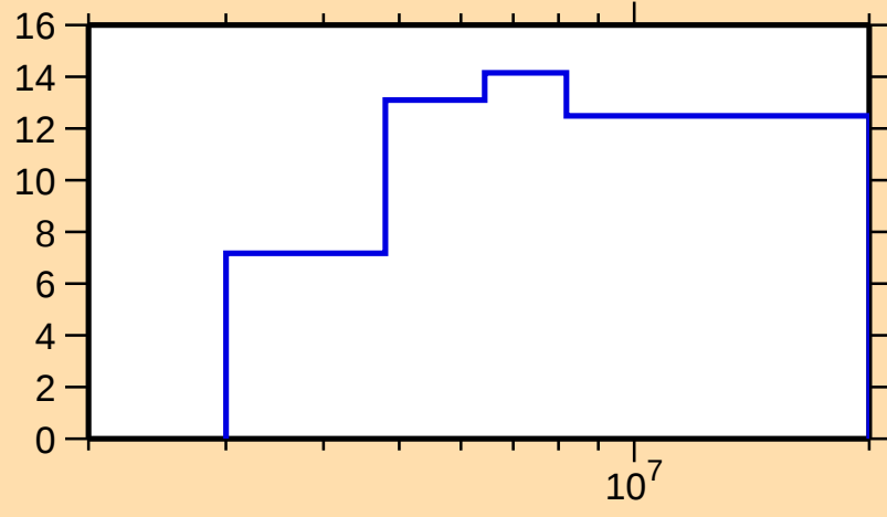
\Delta\sigma/\sigma vs. E for ^{10}\text{C}(\text{n,el.})
