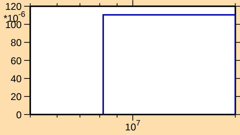
\sigma vs. E for ^{10}\text{C}(n,n\alpha)
