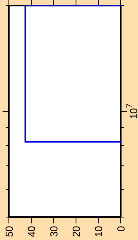
\Delta\sigma/\sigma vs. E for ^{10}\text{C}(n,n\alpha)
