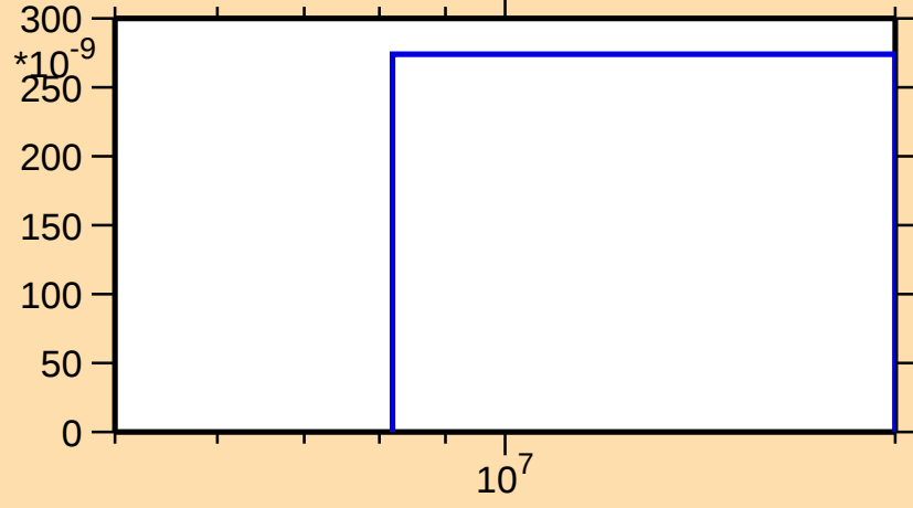
\sigma vs. E for ^{10}\text{C}(\text{mt } 34)
