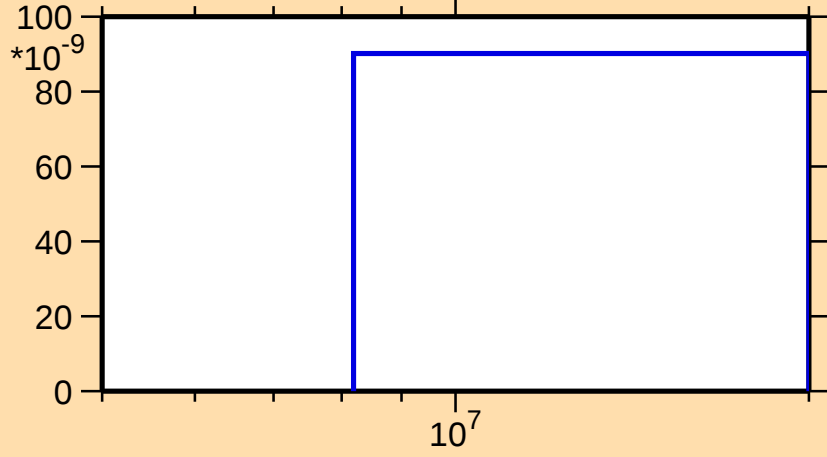
\sigma vs. E for ^{10}\text{C}(\text{n},\text{pt})
