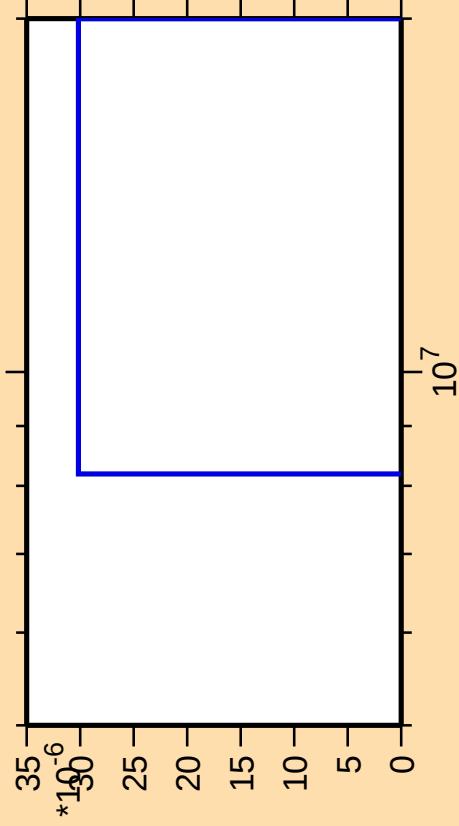
\Delta\sigma/\sigma vs. E for ^{40}\text{Ca}(\text{mt } 34)
