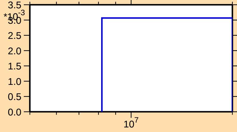
\sigma vs. E for ^{40}\text{Ca}(n,p\alpha)
