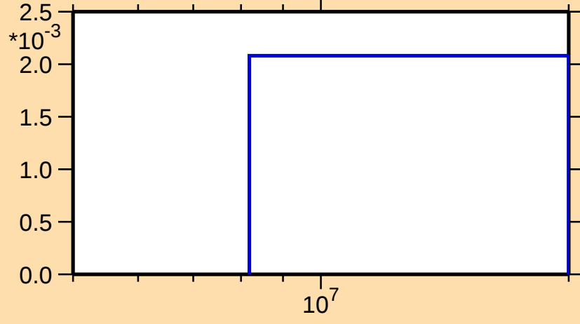
\sigma vs. E for ^{44}\text{Ca}(n,n\alpha)
