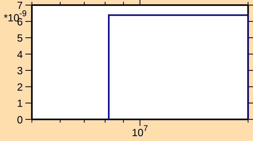
\sigma vs. E for ^{44}\text{Ca}(n,3n)
