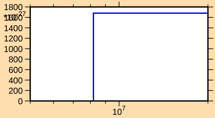
\sigma vs. E for ^{44}\text{Ca}(\text{mt117})
