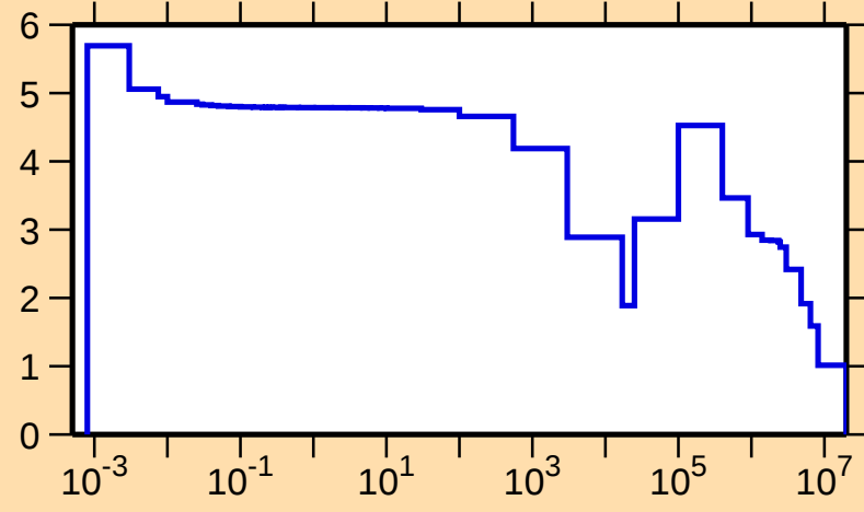
\sigma vs. E for ^{44}\text{Ca}(n,\text{el.})
