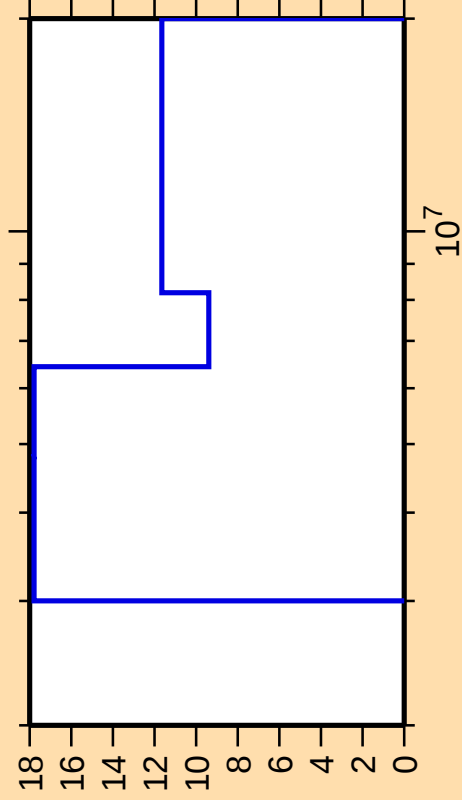
\Delta\sigma/\sigma vs. E for ^{44}\text{Ca}(n,\text{ncont.})
