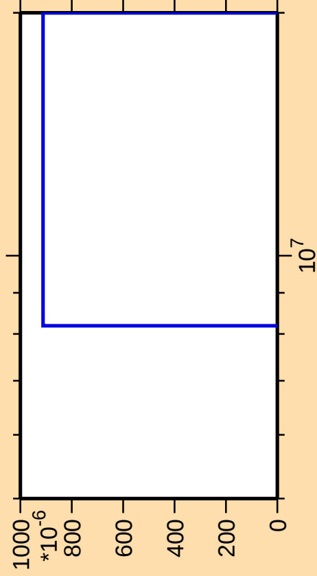
\Delta\sigma/\sigma vs. E for ^{44}\text{Ca}(n,p\alpha)
