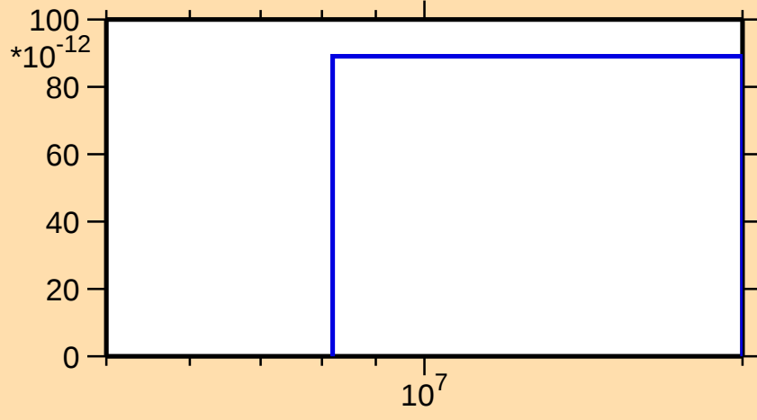
\sigma vs. E for ^{44}\text{Ca}(n,\text{He}3)
