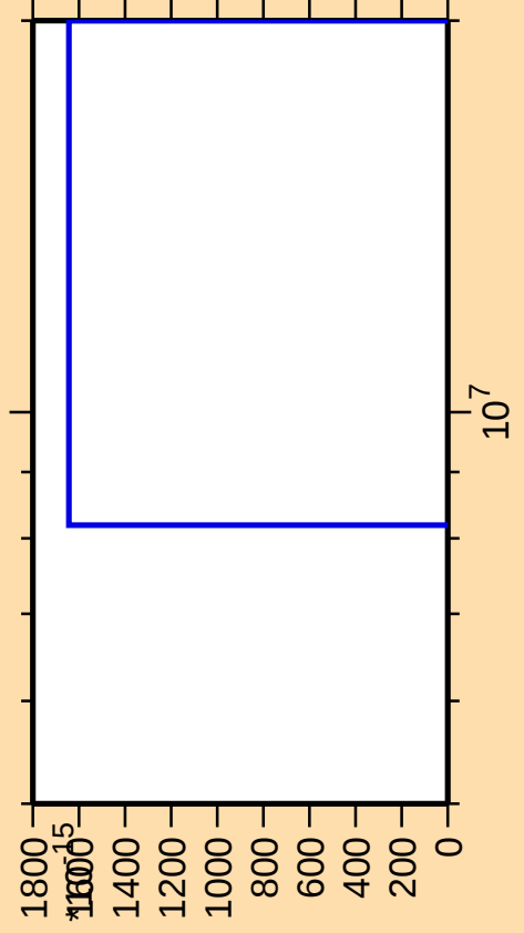
\Delta\sigma/\sigma vs. E for ^{44}\text{Ca}(\text{mt117})
