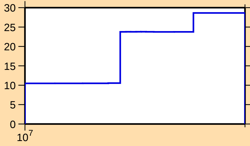
\Delta\sigma/\sigma vs. E for ^{48}\text{Ca}(n,\text{inel.})
