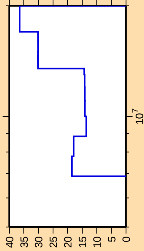
\Delta\sigma/\sigma vs. E for ^{48}\text{Ca}(n,\text{ncont.})
