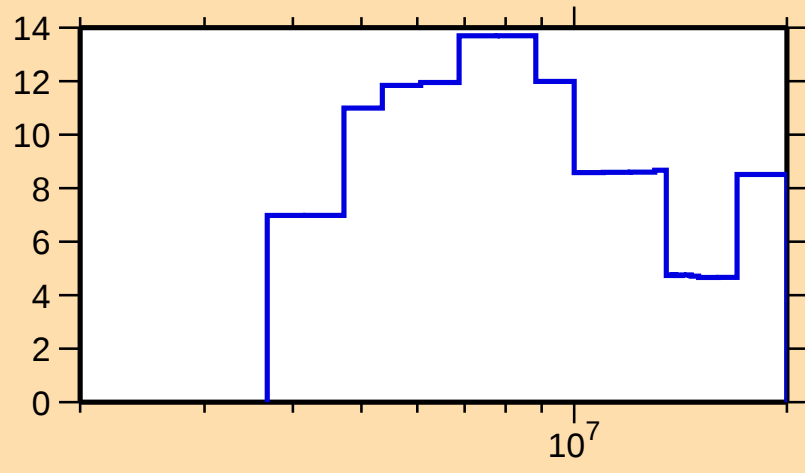
\Delta\sigma/\sigma vs. E for ^{48}\text{Ca}(n,\text{el.})
