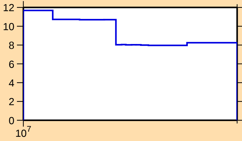
\Delta\sigma/\sigma vs. E for ^{48}\text{Ca}(n,2n)
