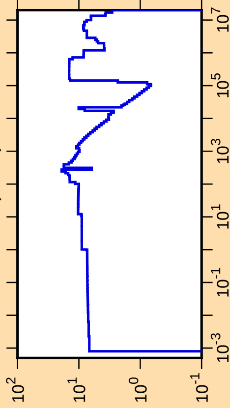
\Delta\sigma/\sigma vs. E for ^{48}\text{Ca}(n,\text{tot.})
