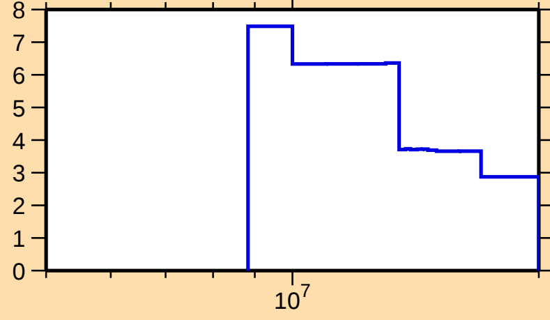
\Delta\sigma/\sigma vs. E for ^{48}\text{Ca}(n,\text{tot.})
