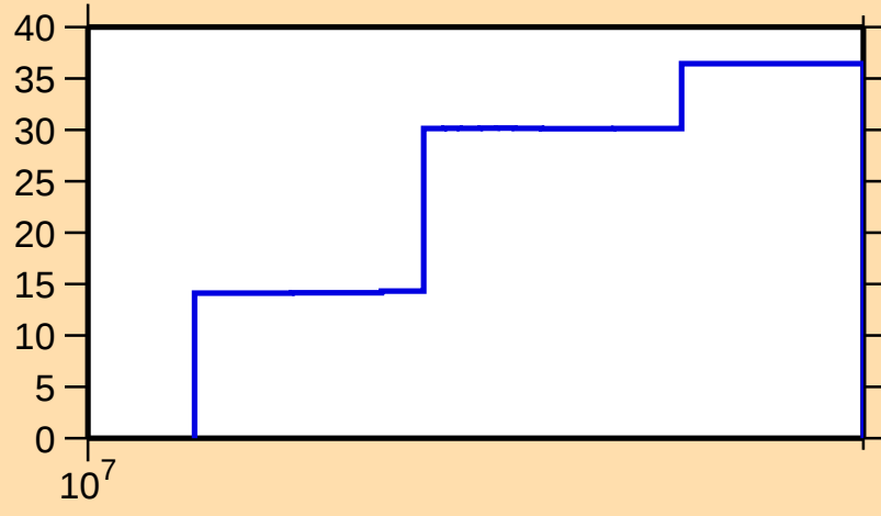
\Delta\sigma/\sigma vs. E for ^{48}\text{Ca}(n,n\text{cont.})
