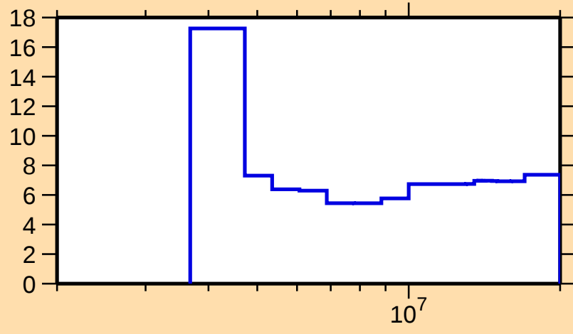
\Delta\sigma/\sigma vs. E for ^{48}\text{Ca}(n,\text{nonel.})
