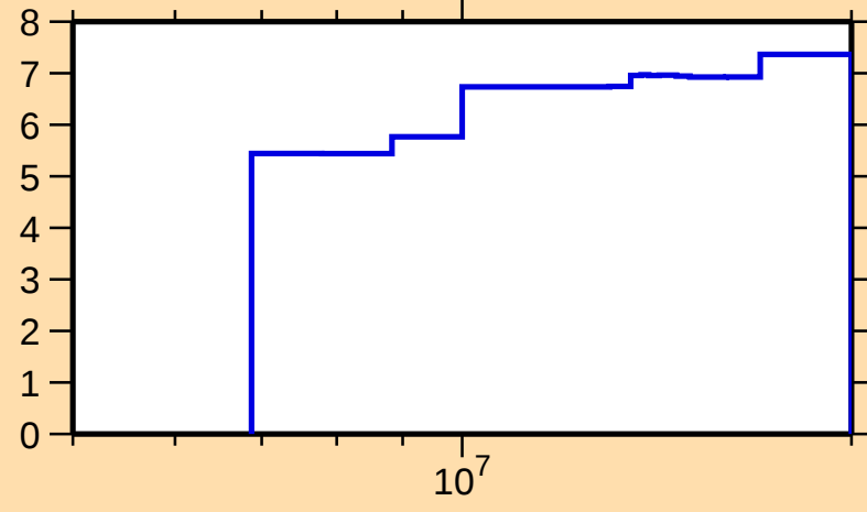
\Delta\sigma/\sigma vs. E for ^{48}\text{Ca}(n,n\text{oncl.})
