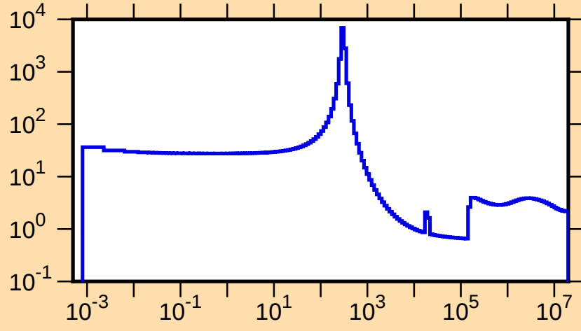
\sigma vs. E for ^{48}\text{Ca}(n,\text{tot.})
