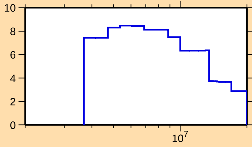
\Delta\sigma/\sigma vs. E for ^{48}\text{Ca}(n,\text{tot.})
