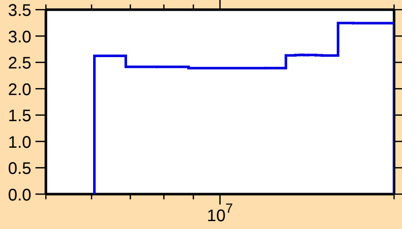
\Delta\sigma/\sigma vs. E for ^{49}\text{Ca}(n,n\text{oncl.})
