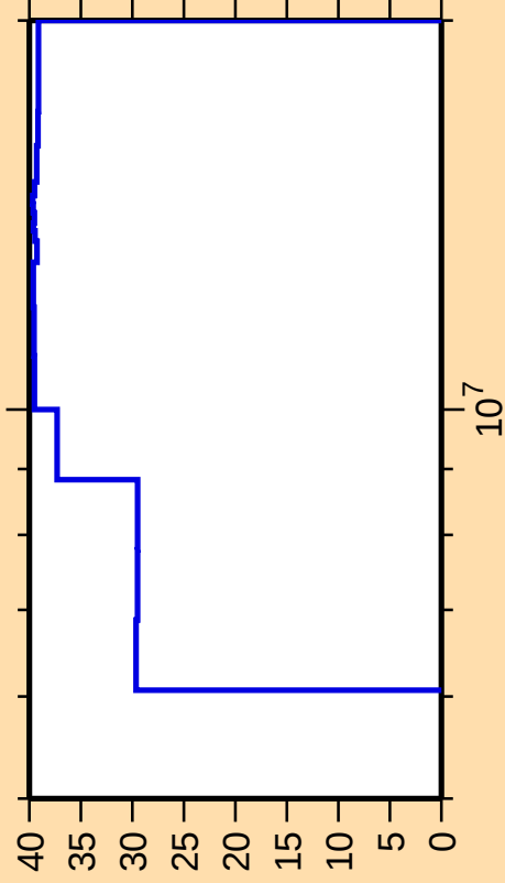
\Delta\sigma/\sigma vs. E for ^{49}\text{Ca}(n,\text{ncont.})
