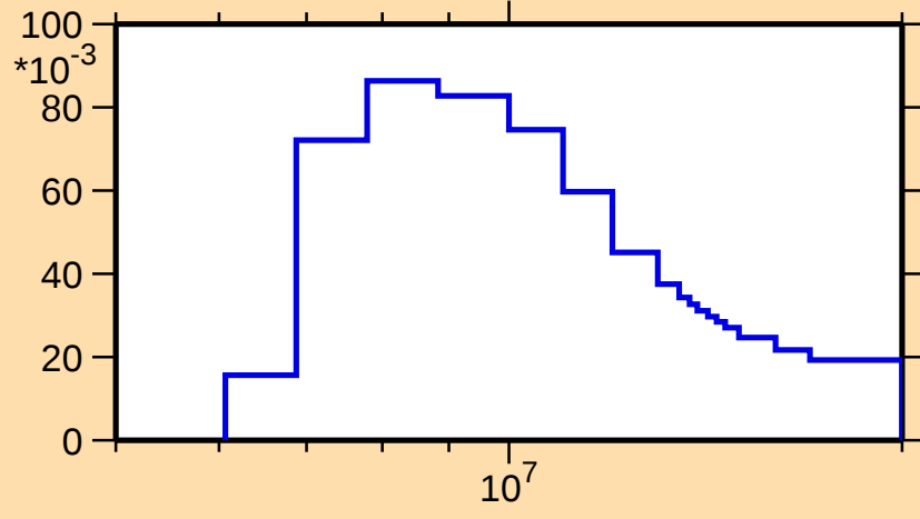
\sigma vs. E for ^{49}\text{Ca}(n,n\text{cont.})
