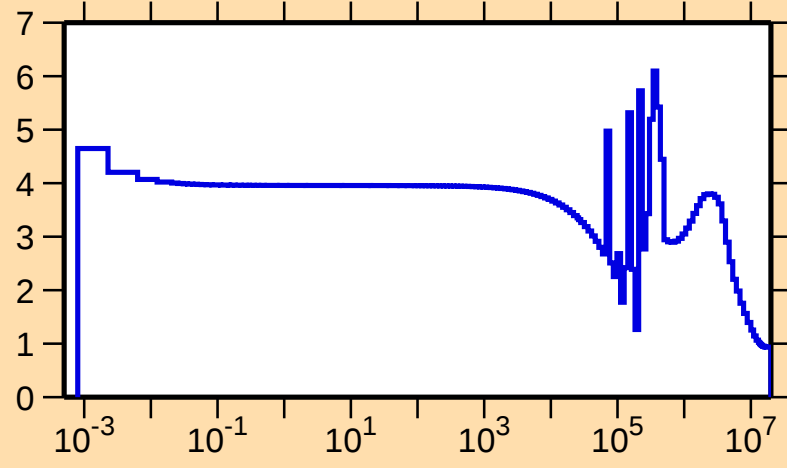
\sigma vs. E for ^{49}\text{Ca}(n,\text{el.})
