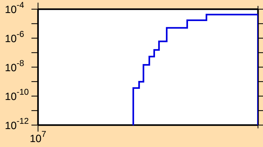
\sigma vs. E for ^{49}\text{Ca}(n,t)
