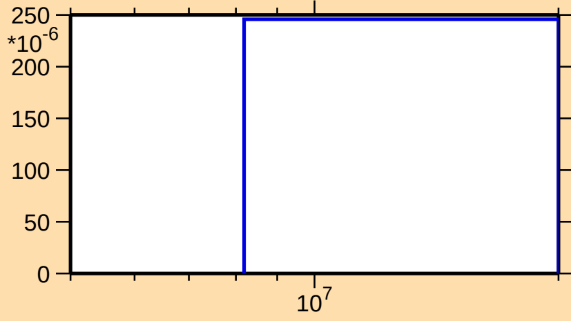
\sigma vs. E for ^{49}\text{Ca}(n,p)
