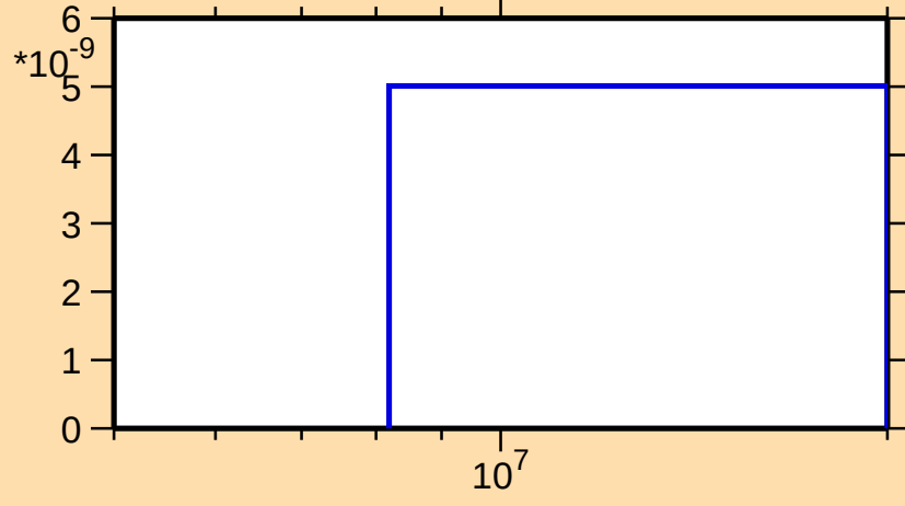
\sigma vs. E for ^{49}\text{Ca}(n,n\alpha)
