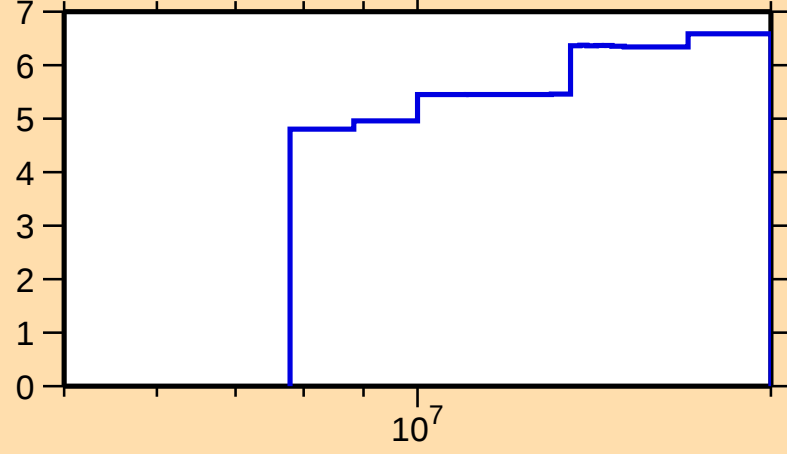
\Delta\sigma/\sigma vs. E for ^{50}\text{Ca}(n,\text{nonel.})
