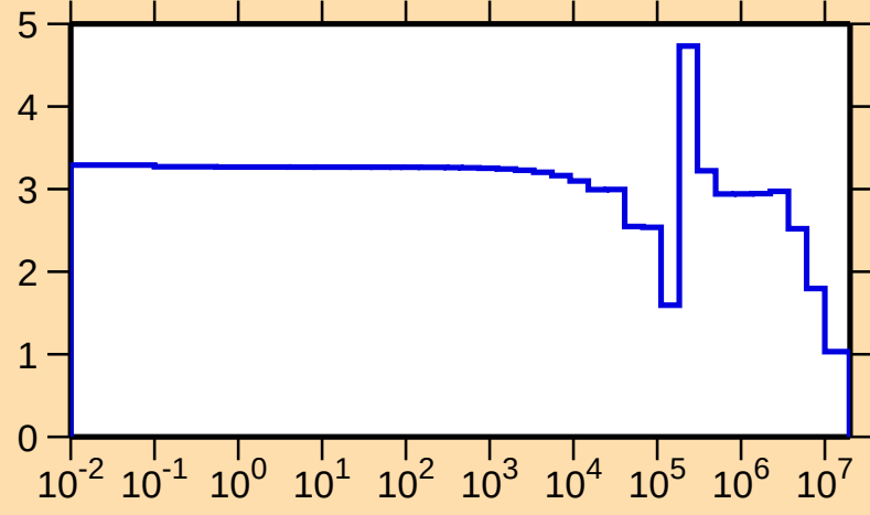
\sigma vs. E for ^{50}\text{Ca}(n,\text{el.})
