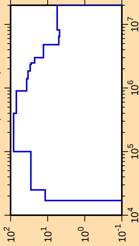
\Delta\sigma/\sigma vs. E for ^{50}\text{Ca}(n,\text{nonel.})
