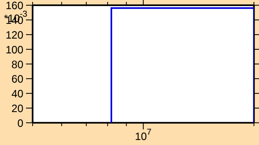
\sigma vs. E for ^{50}\text{Ca}(n,3n)
