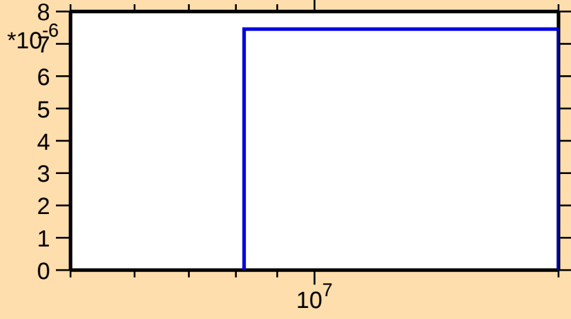
\sigma vs. E for ^{50}\text{Ca}(n,\alpha)
