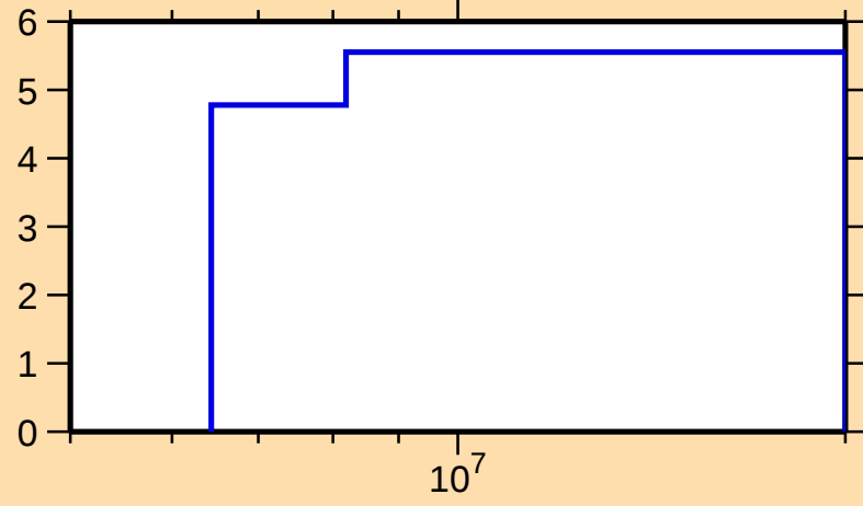
\Delta\sigma/\sigma vs. E for ^{50}\text{Ca}(n,n\text{nonel.})
