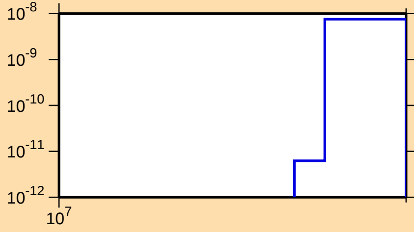
\sigma vs. E for ^{97}\text{Cd}(n,\text{nd})
