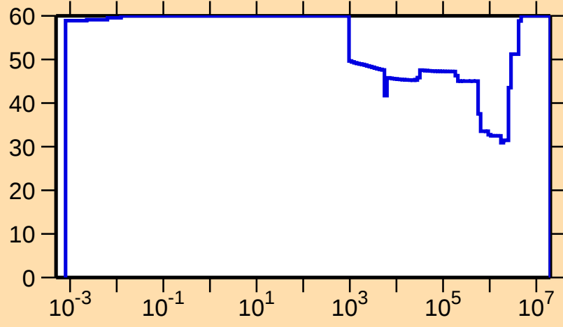
\Delta\sigma/\sigma vs. E for ^{97}\text{Cd}(n,\gamma)
