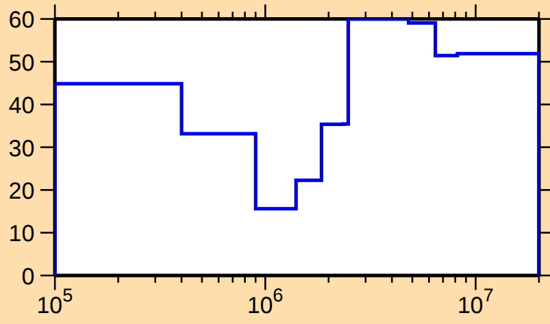
\Delta\sigma/\sigma vs. E for ^{97}\text{Cd}(n,n_1)
