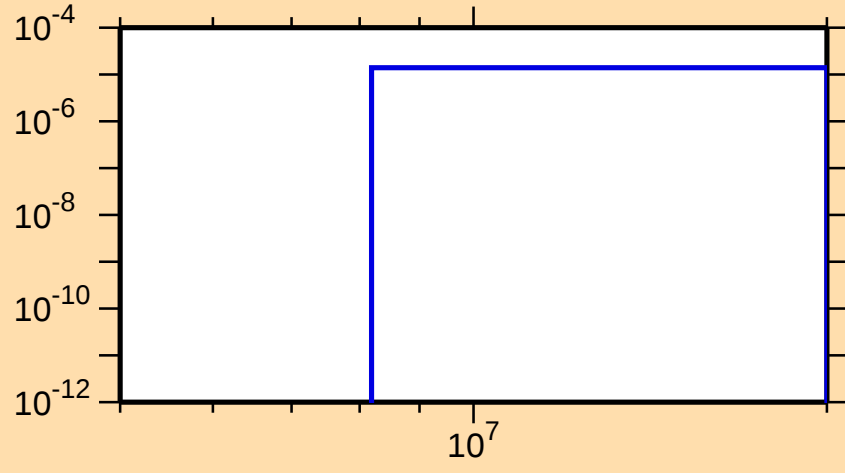
\sigma vs. E for ^{97}\text{Cd}(n,t)
