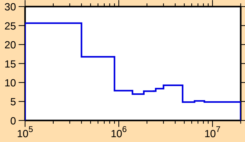
\Delta\sigma/\sigma vs. E for ^{97}\text{Cd}(n,n\text{nonel.})
