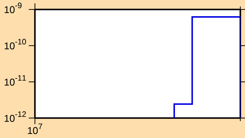
\sigma vs. E for ^{100}\text{Cd}(\text{mt } 34)
