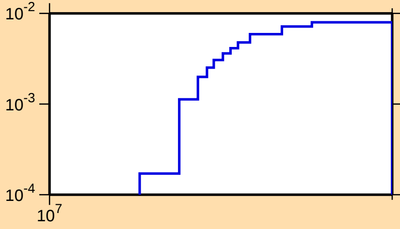
\sigma vs. E for ^{100}\text{Cd}(n,2n)
