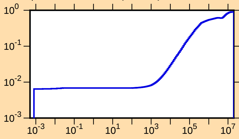
\mu vs. E for ^{105}\text{Cd}(\text{mt251})
