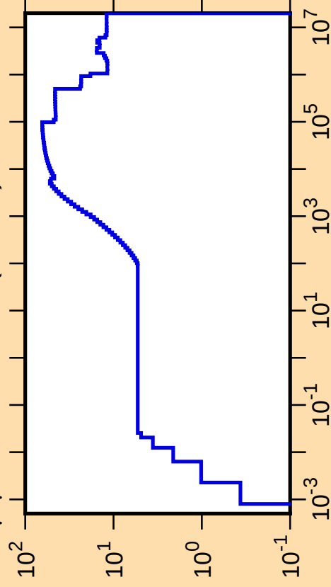
\Delta\mu/\mu vs. E for ^{105}\text{Cd}(\text{mt251})
