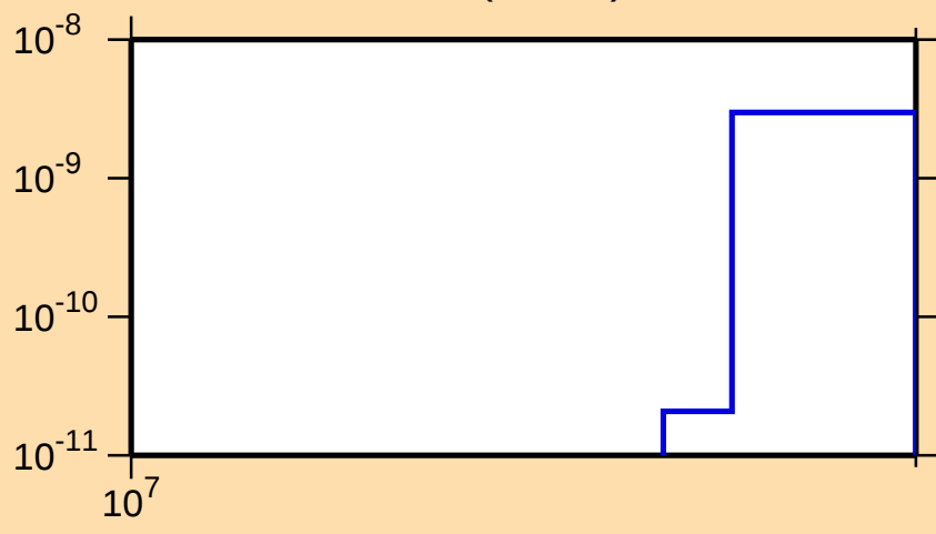
\sigma vs. E for ^{105}\text{Cd}(\text{mt } 45)
