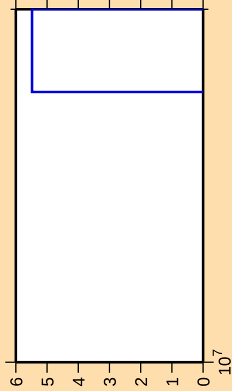
\Delta\sigma/\sigma vs. E for ^{105}\text{Cd}(n,\text{nt})
