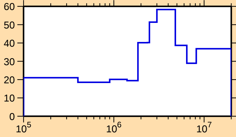
\Delta\sigma/\sigma vs. E for ^{105}\text{Cd}(n,n_1)
