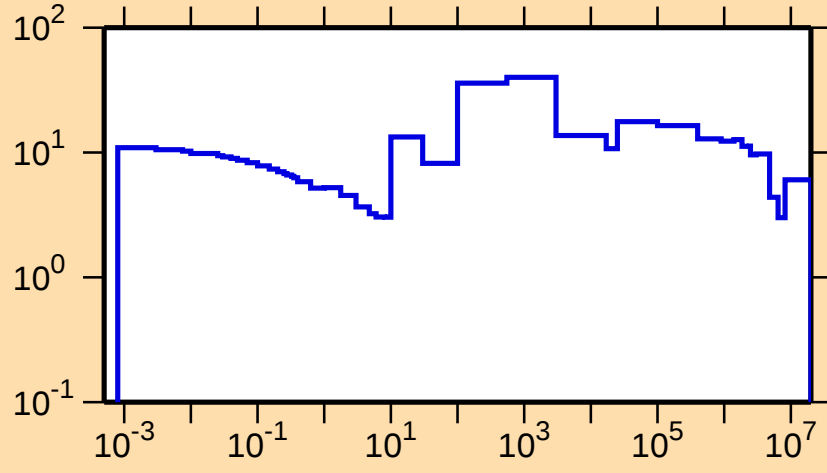
\Delta\sigma/\sigma vs. E for ^{105}\text{Cd}(n,\text{tot.})
