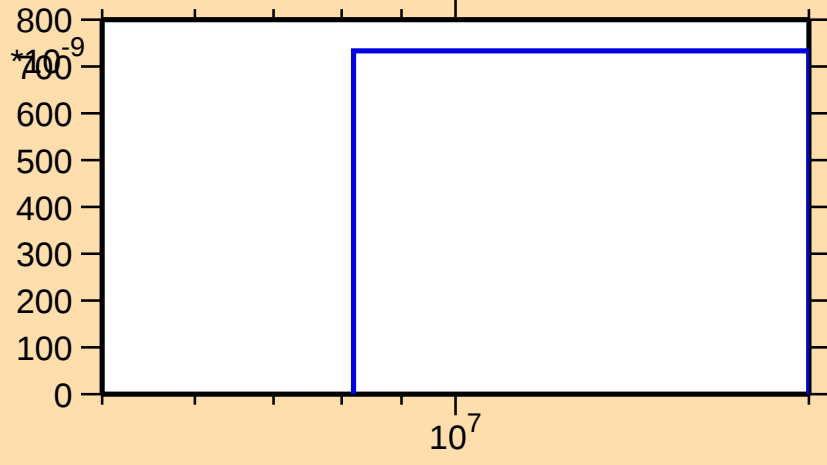
\sigma vs. E for ^{105}\text{Cd}(n,\text{He}3)
