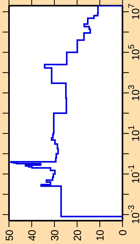
\Delta\sigma/\sigma vs. E for ^{105}\text{Cd}(n,\text{nonel.})
