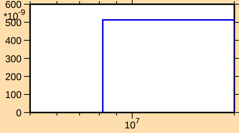
\sigma vs. E for ^{105}\text{Cd}(n,\text{nd})
