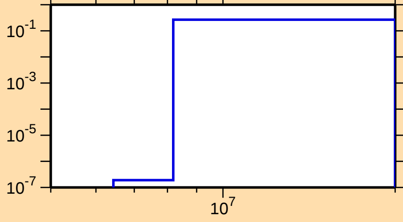
\sigma vs. E for ^{105}\text{Cd}(n,np)
