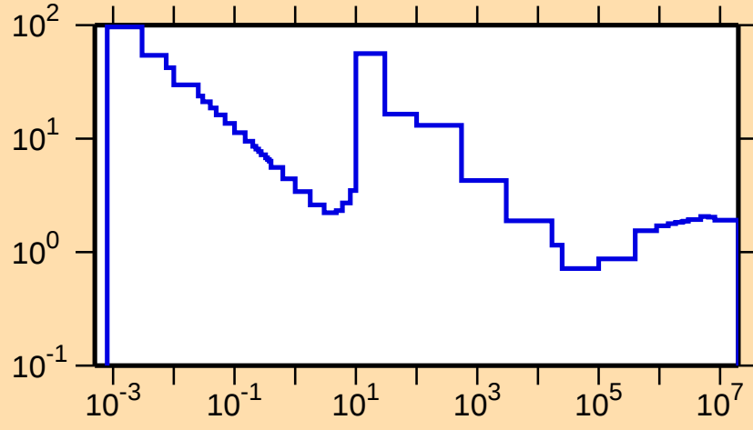
\sigma vs. E for ^{105}\text{Cd}(n,\text{nonel.})
