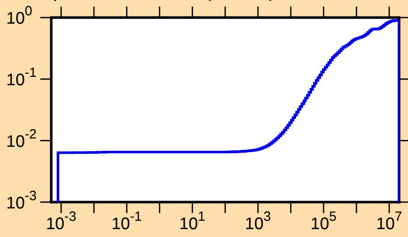
\mu vs. E for ^{106}\text{Cd}(\text{mt251})
