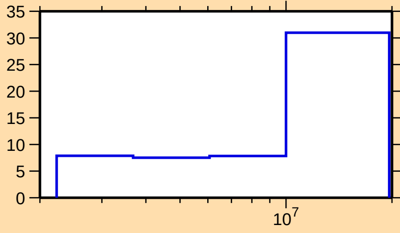
\Delta\sigma/\sigma vs. E for ^{106}\text{Cd}(n,n\text{cont.})
