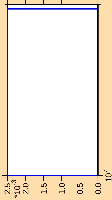
\Delta\sigma/\sigma vs. E for ^{106}\text{Cd}(n,nt)
