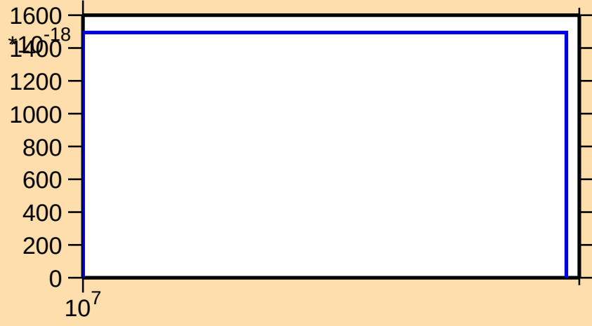
\sigma vs. E for ^{106}\text{Cd}(n,nt)
