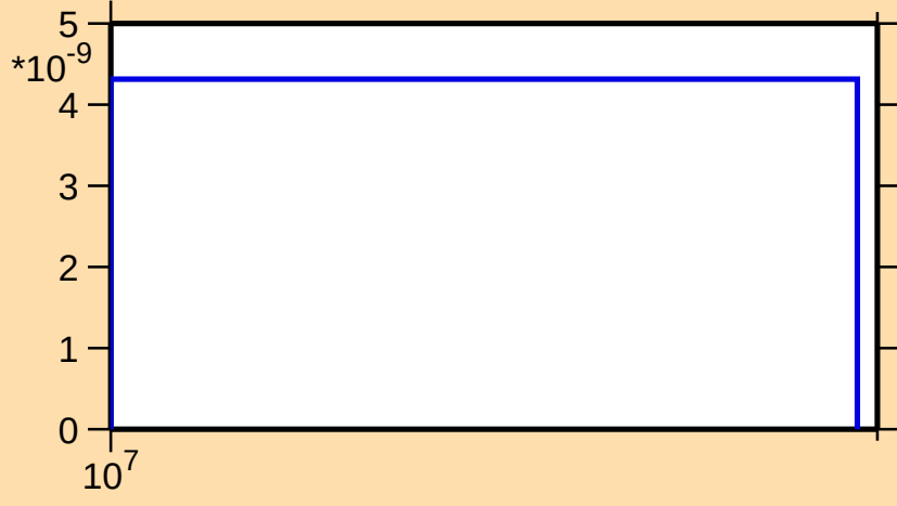
\sigma vs. E for ^{106}\text{Cd}(n,\text{pd})
