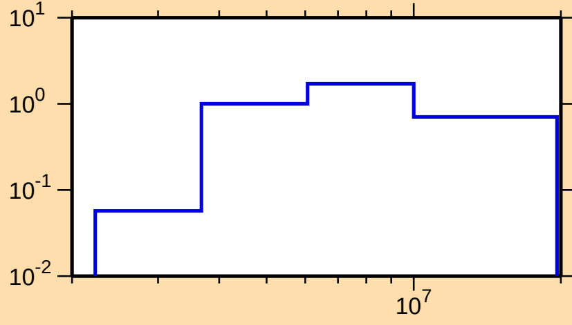
\sigma vs. E for ^{106}\text{Cd}(n,n\text{cont.})
