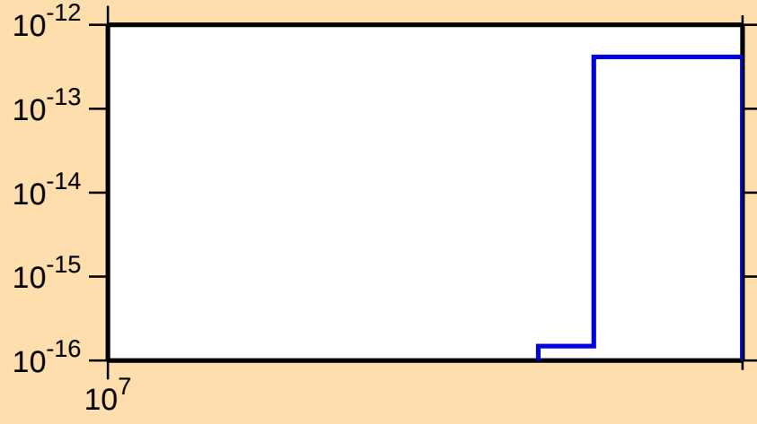
\sigma vs. E for ^{107}\text{Cd}(\text{mt } 45)
