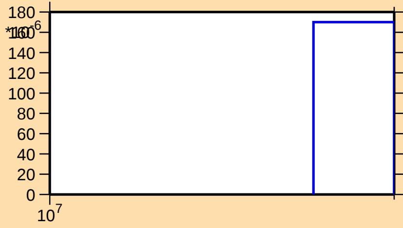
\sigma vs. E for ^{107}\text{Cd}(n,3n)
