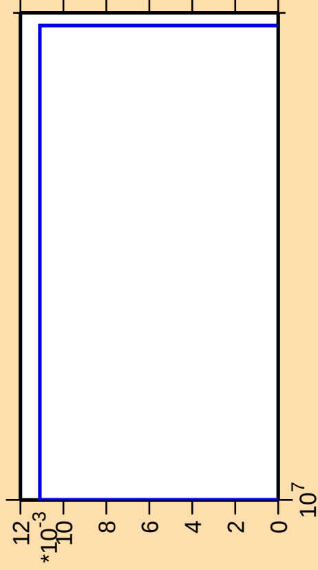
\Delta\sigma/\sigma vs. E for ^{107}\text{Cd}(\text{mt } 45)
