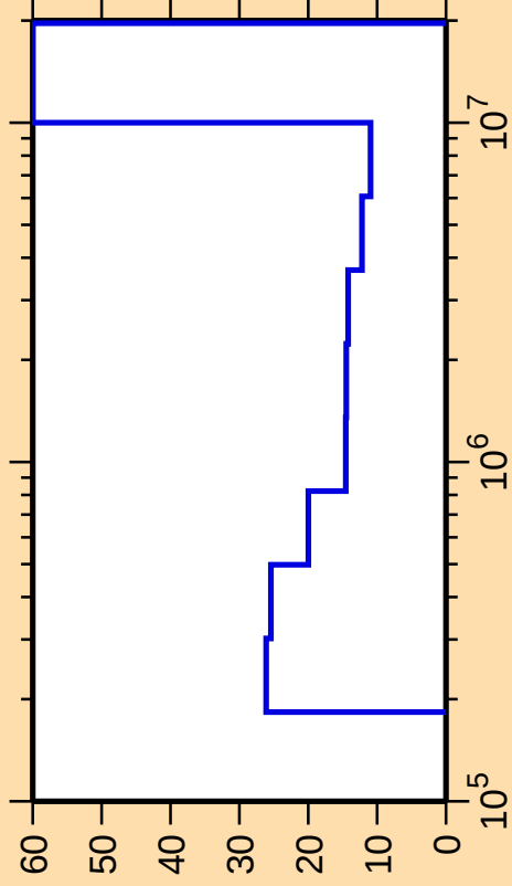
\Delta\sigma/\sigma vs. E for ^{107}\text{Cd}(n,\text{inel.})
