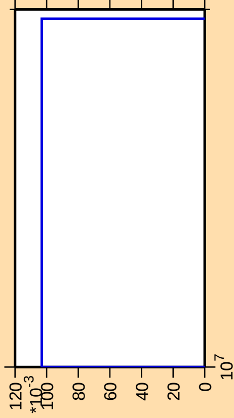
\Delta\sigma/\sigma vs. E for ^{107}\text{Cd}(n,\text{nt})
