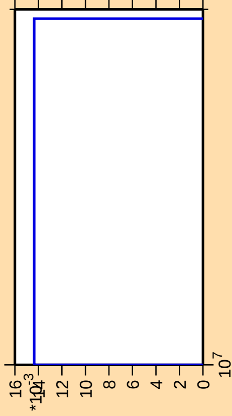
\Delta\sigma/\sigma vs. E for ^{107}\text{Cd}(\text{mt117})
