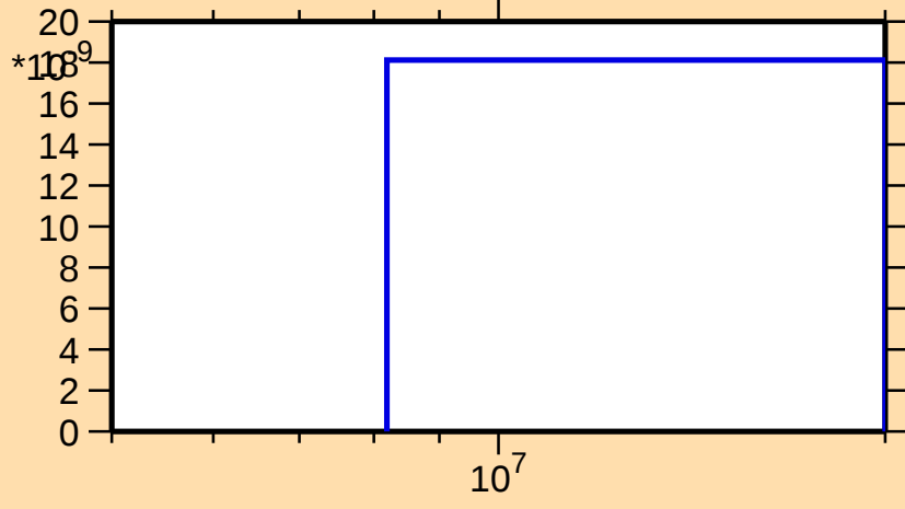
\sigma vs. E for ^{107}\text{Cd}(n,\text{He}3)
