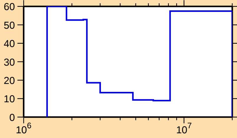
\Delta\sigma/\sigma vs. E for ^{107}\text{Cd}(n,n\text{cont.})
