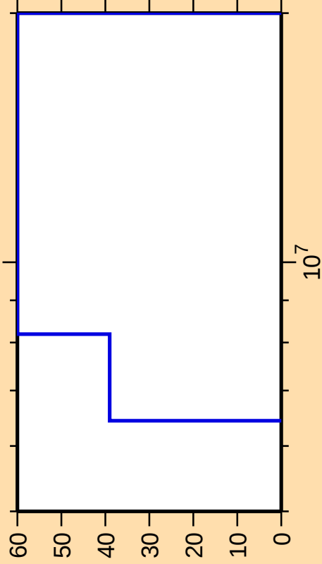
\Delta\sigma/\sigma vs. E for ^{107}\text{Cd}(n,\alpha)
