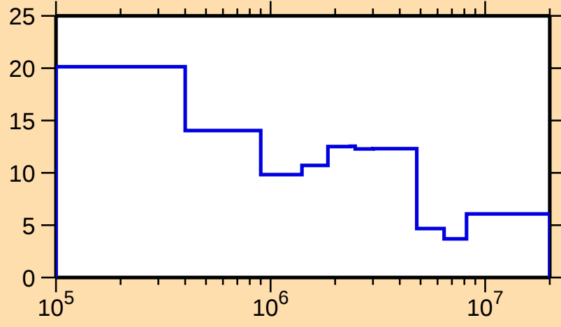
\Delta\sigma/\sigma vs. E for ^{107}\text{Cd}(n,\text{tot.})
