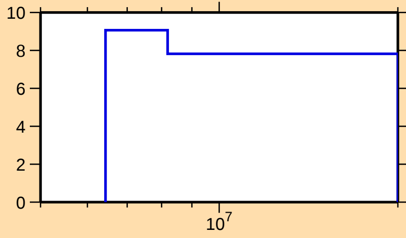
\Delta\sigma/\sigma vs. E for ^{107}\text{Cd}(n,\text{nonel.})
