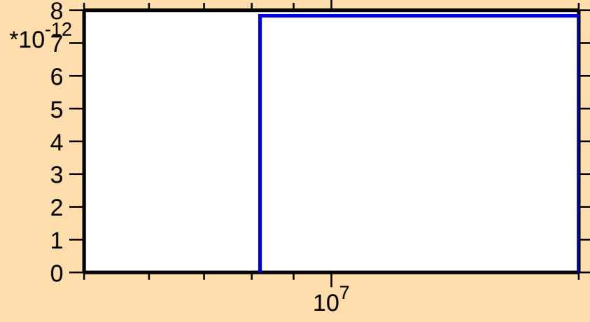
\sigma vs. E for ^{107}\text{Cd}(n,\text{pd})
