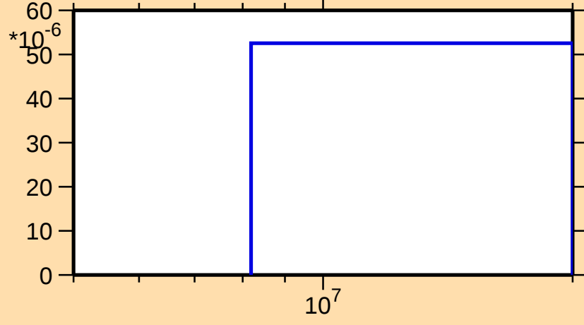
\sigma vs. E for ^{107}\text{Cd}(n,t)
