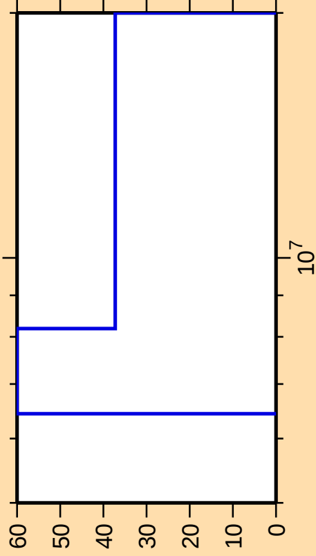
\Delta\sigma/\sigma vs. E for ^{107}\text{Cd}(n,n_1)
