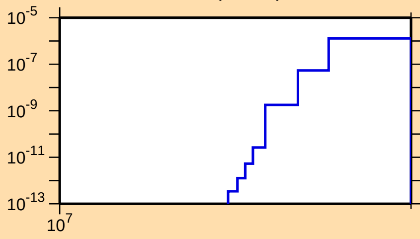
\sigma vs. E for ^{109}\text{Cd}(n,2n\alpha)
