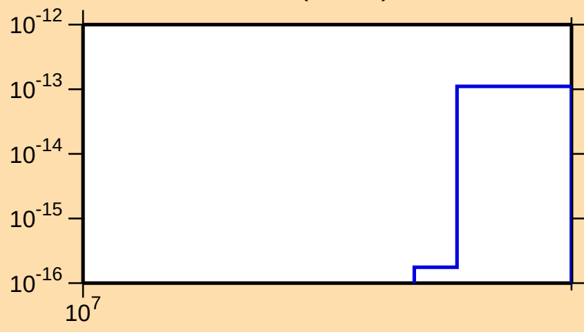
\sigma vs. E for ^{109}\text{Cd} (mt 34)
