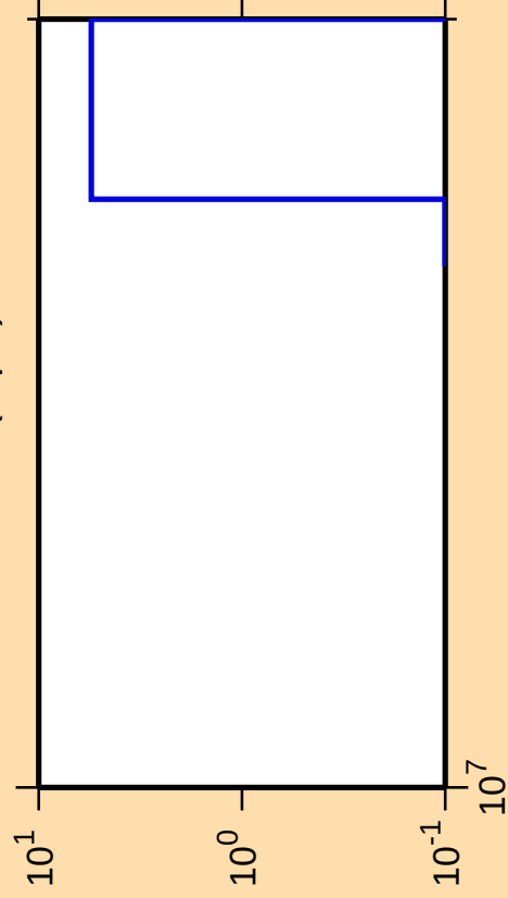
\Delta\sigma/\sigma vs. E for ^{109}\text{Cd}(n,\text{pd})
