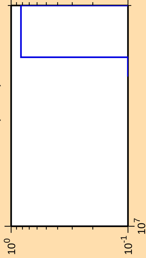
\Delta\sigma/\sigma vs. E for ^{109}\text{Cd} (mt 34)
