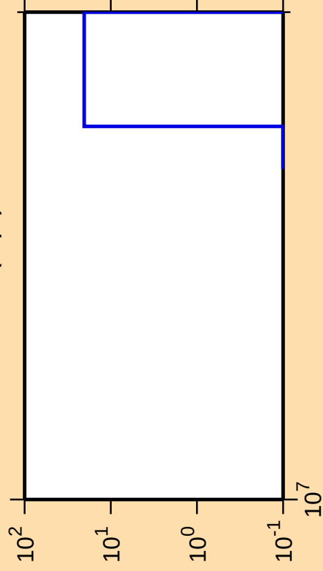
\Delta\sigma/\sigma vs. E for ^{109}\text{Cd}(n,\text{pt})
