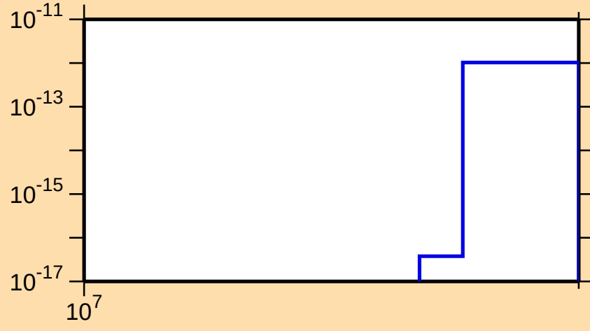
\sigma vs. E for ^{109}\text{Cd}(n,\text{pd})
