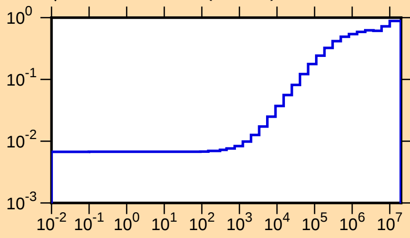
\mu vs. E for ^{109}\text{Cd}(\text{mt251})
