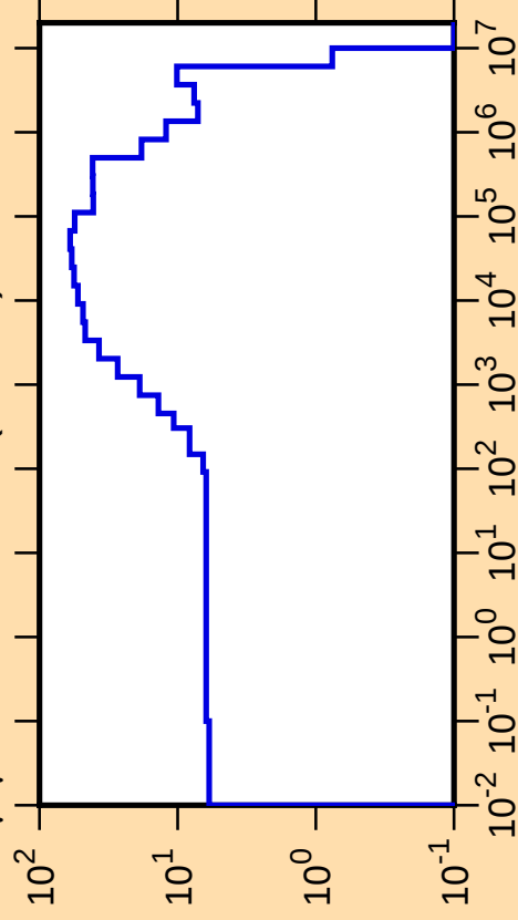
\Delta\mu/\mu vs. E for ^{109}\text{Cd}(\text{mt251})
