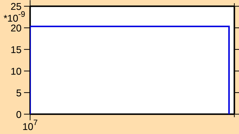
\sigma vs. E for ^{109}\text{Cd}(n,2np)
