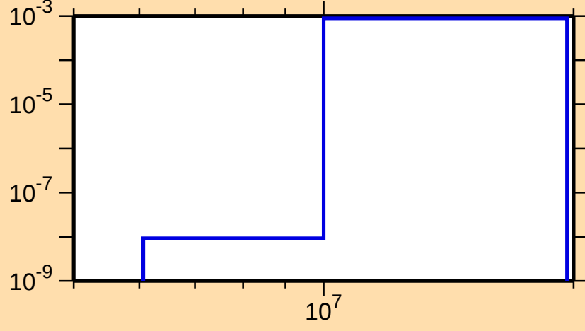
\sigma vs. E for ^{109}\text{Cd}(n,n\alpha)
