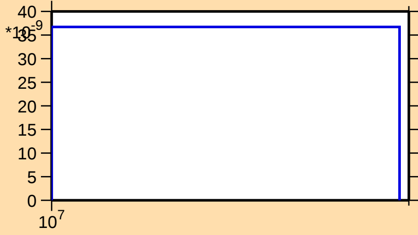
\sigma vs. E for ^{109}\text{Cd}(n,\text{nd})
