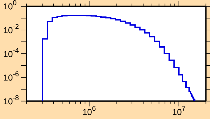
\sigma vs. E for ^{121}\text{Cd}(n,n_4)
