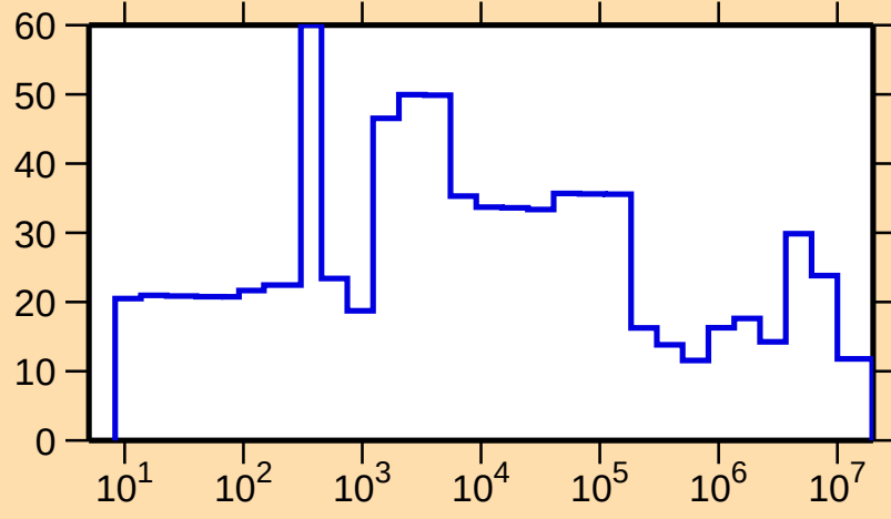
\Delta\sigma/\sigma vs. E for ^{121}\text{Cd}(n,\text{el.})
