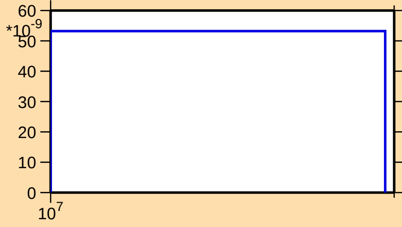
\sigma vs. E for ^{121}\text{Cd}(n,n\alpha)
