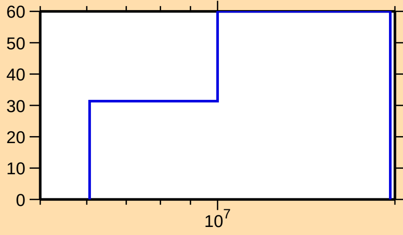
\Delta\sigma/\sigma vs. E for ^{121}\text{Cd}(n,n\text{cont.})
