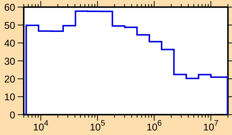
\Delta\sigma/\sigma vs. E for ^{121}\text{Cd}(n,\text{nonel.})
