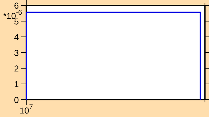
\sigma vs. E for ^{121}\text{Cd}(n,d)
