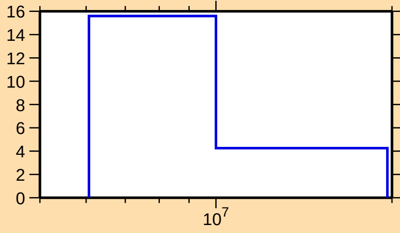
\Delta\sigma/\sigma vs. E for ^{121}\text{Cd}(n,\text{tot.})
