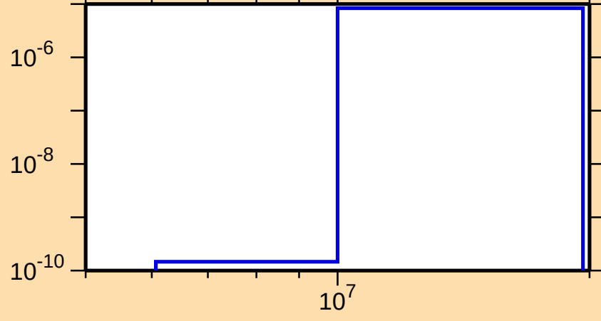
\sigma vs. E for ^{121}\text{Cd}(n,\alpha)
