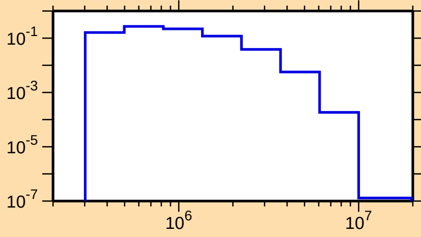
\sigma vs. E for ^{121}\text{Cd}(n,n_3)
