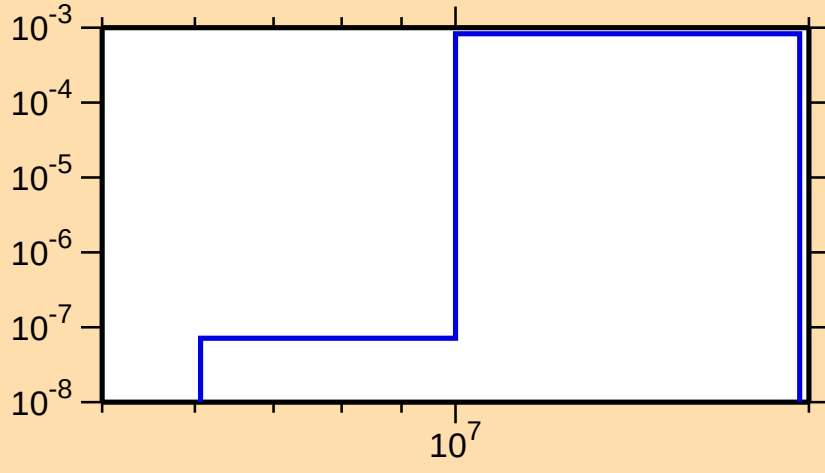
\sigma vs. E for ^{121}\text{Cd}(n,p)
