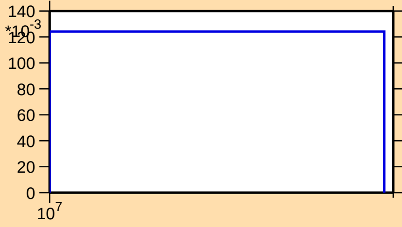
\sigma vs. E for ^{121}\text{Cd}(n,3n)
